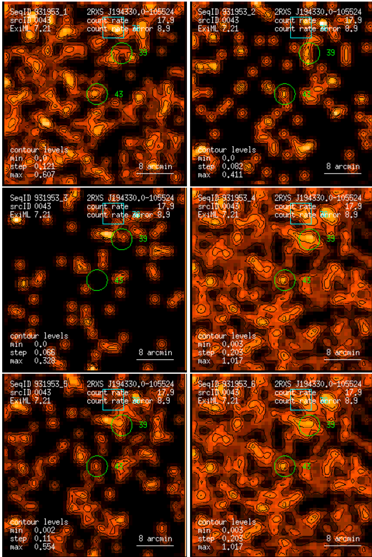
Figure 43: RASS 931953: detection 0043: band rate images, Gaussian filter: (1) PSPC channels 11 – 41, (2) 52 – 90, (3) 91 – 201, (4) 11 – 235, (5) 52 – 201, (6) 11 – 201. Broad band rates in counts/ks. Band rate contour levels in counts/ks/arcmin 2 .
