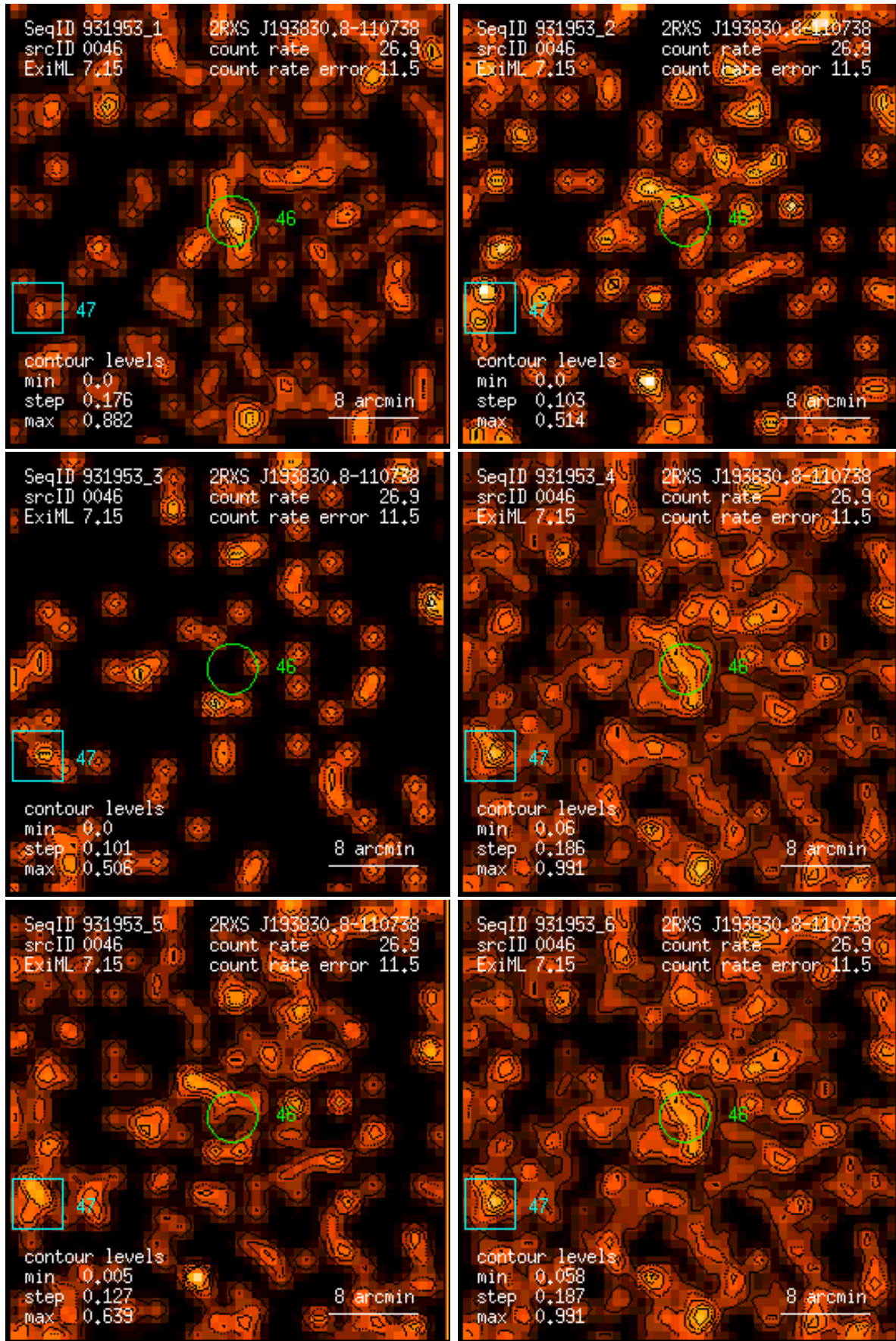
Figure 46: RASS 931953: detection 0046: band rate images, Gaussian filter: (1) PSPC channels 11 – 41, (2) 52 – 90, (3) 91 – 201, (4) 11 – 235, (5) 52 – 201, (6) 11 – 201. Broad band rates in counts/ks. Band rate contour levels in counts/ks/arcmin 2 .
