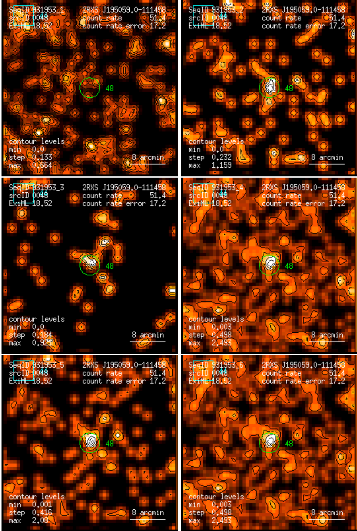
Figure 48: RASS 931953: detection 0048: band rate images, Gaussian filter: (1) PSPC channels 11 – 41, (2) 52 – 90, (3) 91 – 201, (4) 11 – 235, (5) 52 – 201, (6) 11 – 201. Broad band rates in counts/ks. Band rate contour levels in counts/ks/arcmin 2 .
