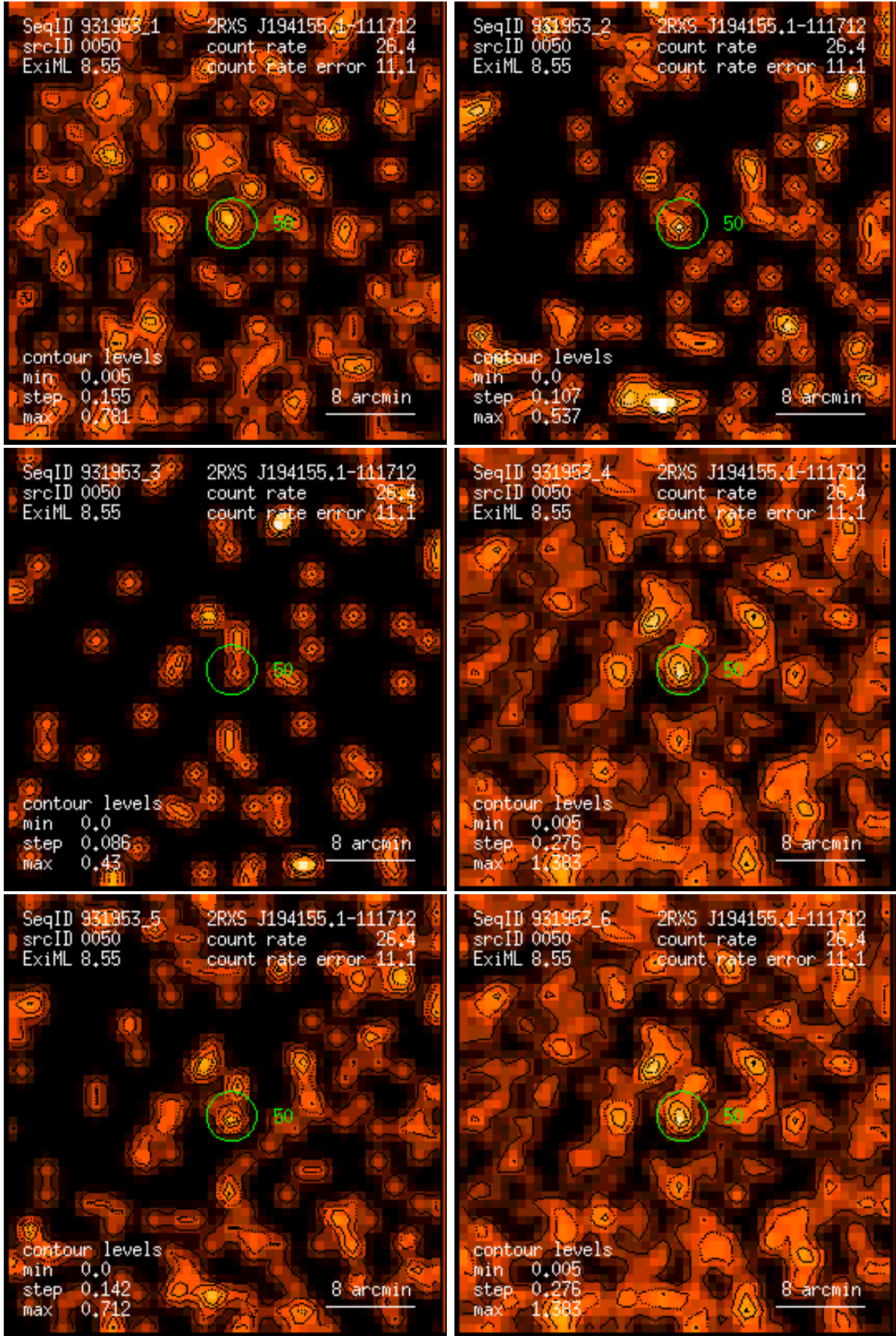
Figure 50: RASS 931953: detection 0050: band rate images, Gaussian filter: (1) PSPC channels 11 – 41, (2) 52 – 90, (3) 91 – 201, (4) 11 – 235, (5) 52 – 201, (6) 11 – 201. Broad band rates in counts/ks. Band rate contour levels in counts/ks/arcmin 2 .
