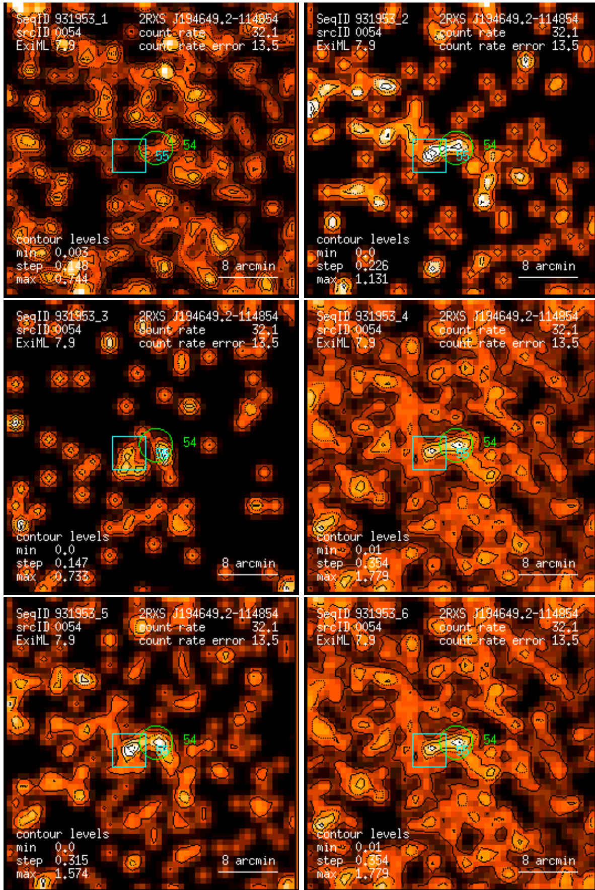
Figure 54: RASS 931953: detection 0054: band rate images, Gaussian filter: (1) PSPC channels 11 – 41, (2) 52 – 90, (3) 91 – 201, (4) 11 – 235, (5) 52 – 201, (6) 11 – 201. Broad band rates in counts/ks. Band rate contour levels in counts/ks/arcmin 2 .
