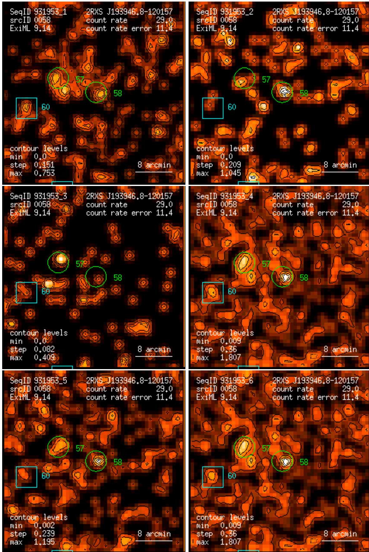
Figure 58: RASS 931953: detection 0058: band rate images, Gaussian filter: (1) PSPC channels 11 – 41, (2) 52 – 90, (3) 91 – 201, (4) 11 – 235, (5) 52 – 201, (6) 11 – 201. Broad band rates in counts/ks. Band rate contour levels in counts/ks/arcmin 2 .
