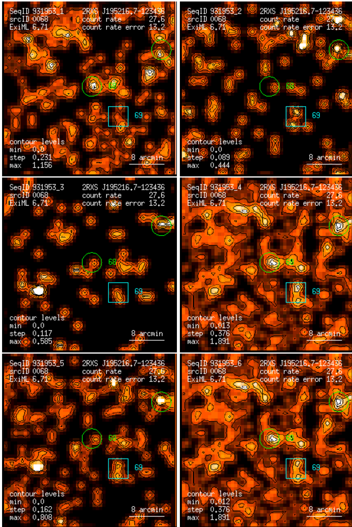
Figure 68: RASS 931953: detection 0068: band rate images, Gaussian filter: (1) PSPC channels 11 – 41, (2) 52 – 90, (3) 91 – 201, (4) 11 – 235, (5) 52 – 201, (6) 11 – 201. Broad band rates in counts/ks. Band rate contour levels in counts/ks/arcmin 2 .
