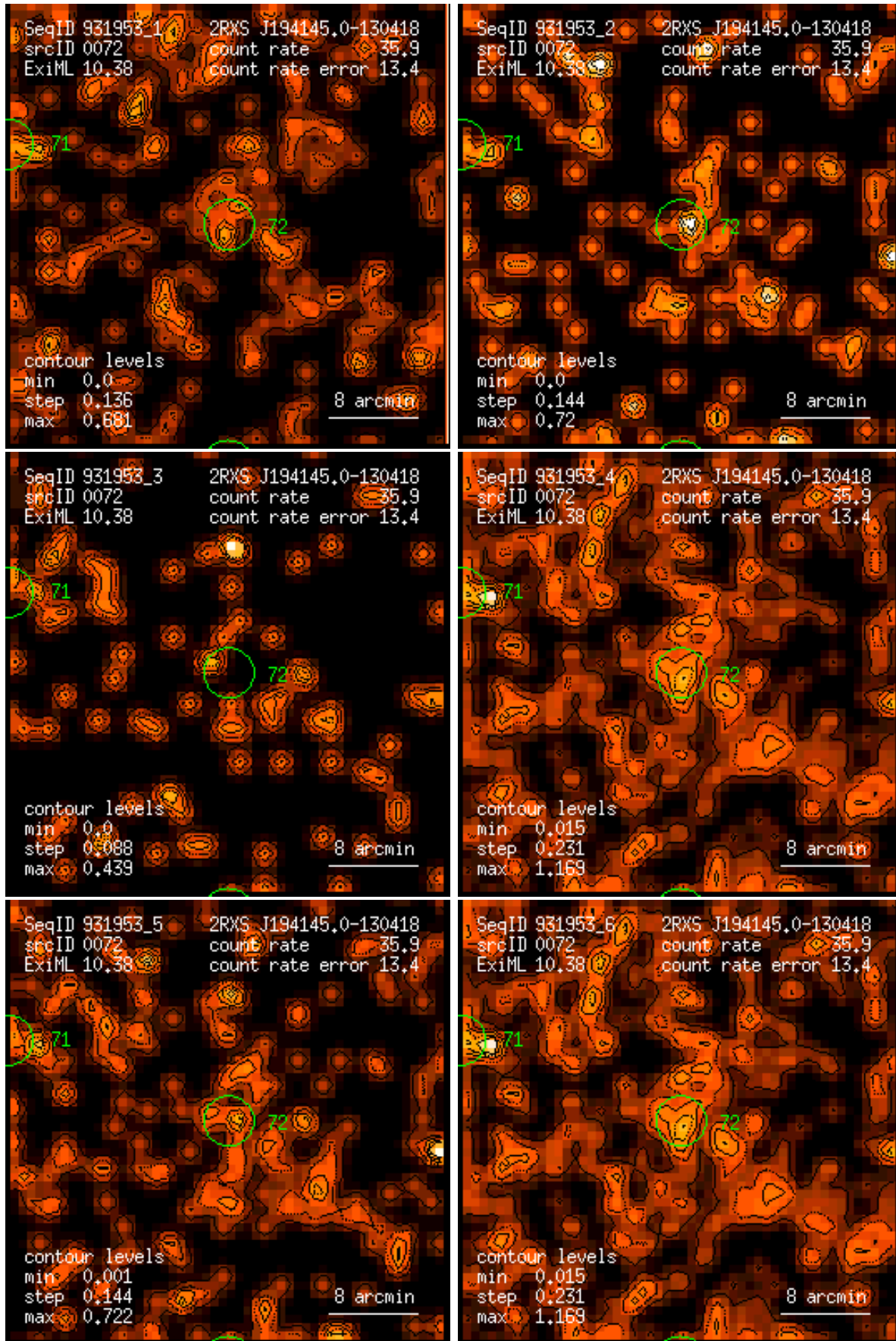
Figure 72: RASS 931953: detection 0072: band rate images, Gaussian filter: (1) PSPC channels 11 – 41, (2) 52 – 90, (3) 91 – 201, (4) 11 – 235, (5) 52 – 201, (6) 11 – 201. Broad band rates in counts/ks. Band rate contour levels in counts/ks/arcmin 2 .
