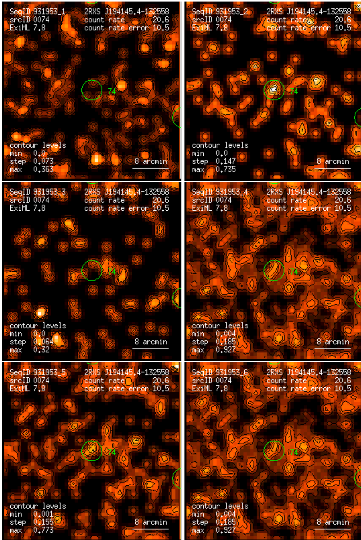
Figure 74: RASS 931953: detection 0074: band rate images, Gaussian filter: (1) PSPC channels 11 – 41, (2) 52 – 90, (3) 91 – 201, (4) 11 – 235, (5) 52 – 201, (6) 11 – 201. Broad band rates in counts/ks. Band rate contour levels in counts/ks/arcmin 2 .
