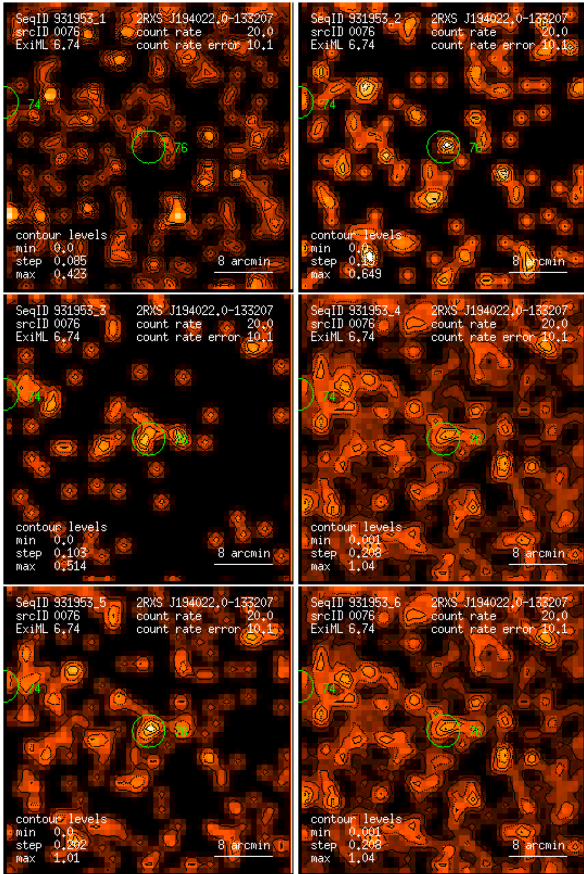
Figure 76: RASS 931953: detection 0076: band rate images, Gaussian filter: (1) PSPC channels 11 – 41, (2) 52 – 90, (3) 91 – 201, (4) 11 – 235, (5) 52 – 201, (6) 11 – 201. Broad band rates in counts/ks. Band rate contour levels in counts/ks/arcmin 2 .
