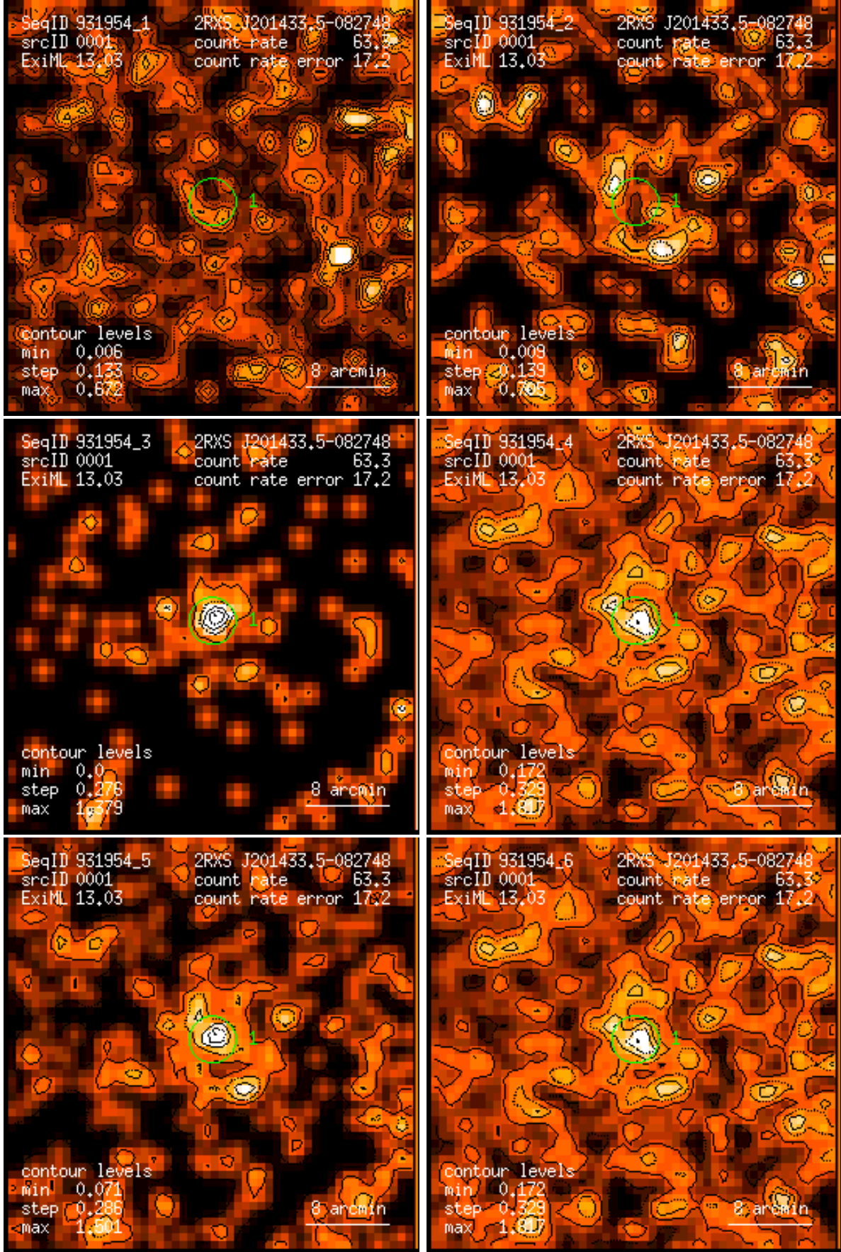
Figure 1: RASS 931954: detection 0001: band rate images, Gaussian filter: (1) PSPC channels 11 – 41, (2) 52 – 90, (3) 91 – 201, (4) 11 – 235, (5) 52 – 201, (6) 11 – 201. Broad band rates in counts/ks. Band rate contour levels in counts/ks/arcmin 2 .
