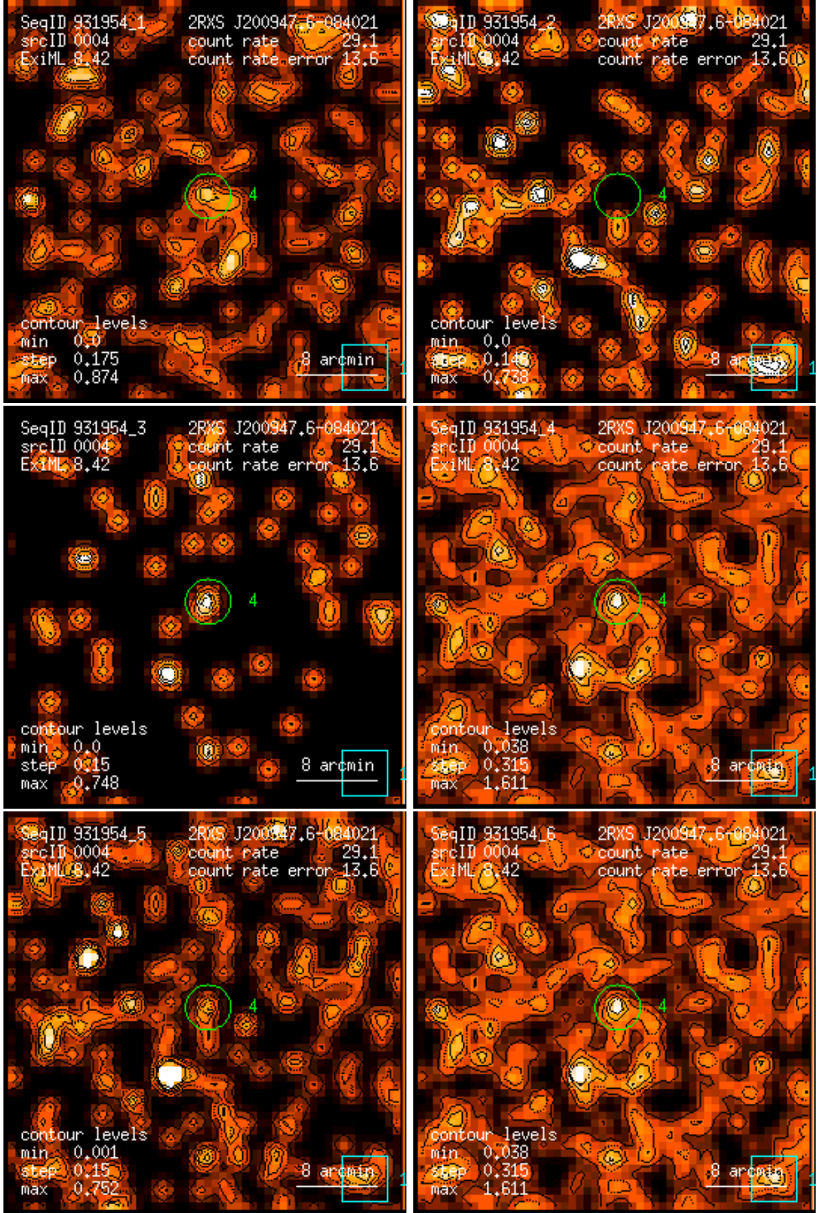
Figure 4: RASS 931954: detection 0004: band rate images, Gaussian filter: (1) PSPC channels 11 – 41, (2) 52 – 90, (3) 91 – 201, (4) 11 – 235, (5) 52 – 201, (6) 11 – 201. Broad band rates in counts/ks. Band rate contour levels in counts/ks/arcmin 2 .
