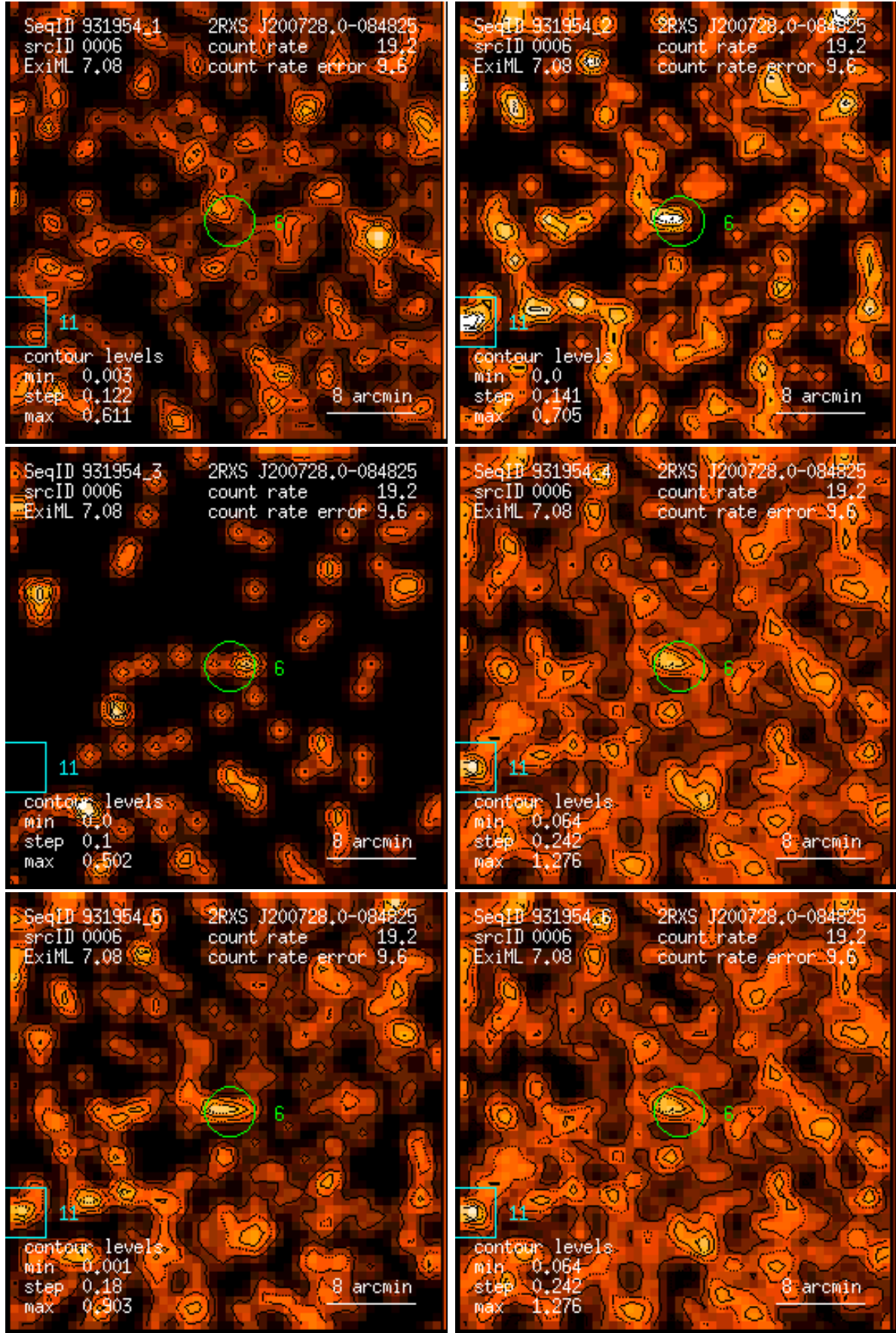
Figure 6: RASS 931954: detection 0006: band rate images, Gaussian filter: (1) PSPC channels 11 – 41, (2) 52 – 90, (3) 91 – 201, (4) 11 – 235, (5) 52 – 201, (6) 11 – 201. Broad band rates in counts/ks. Band rate contour levels in counts/ks/arcmin 2 .
