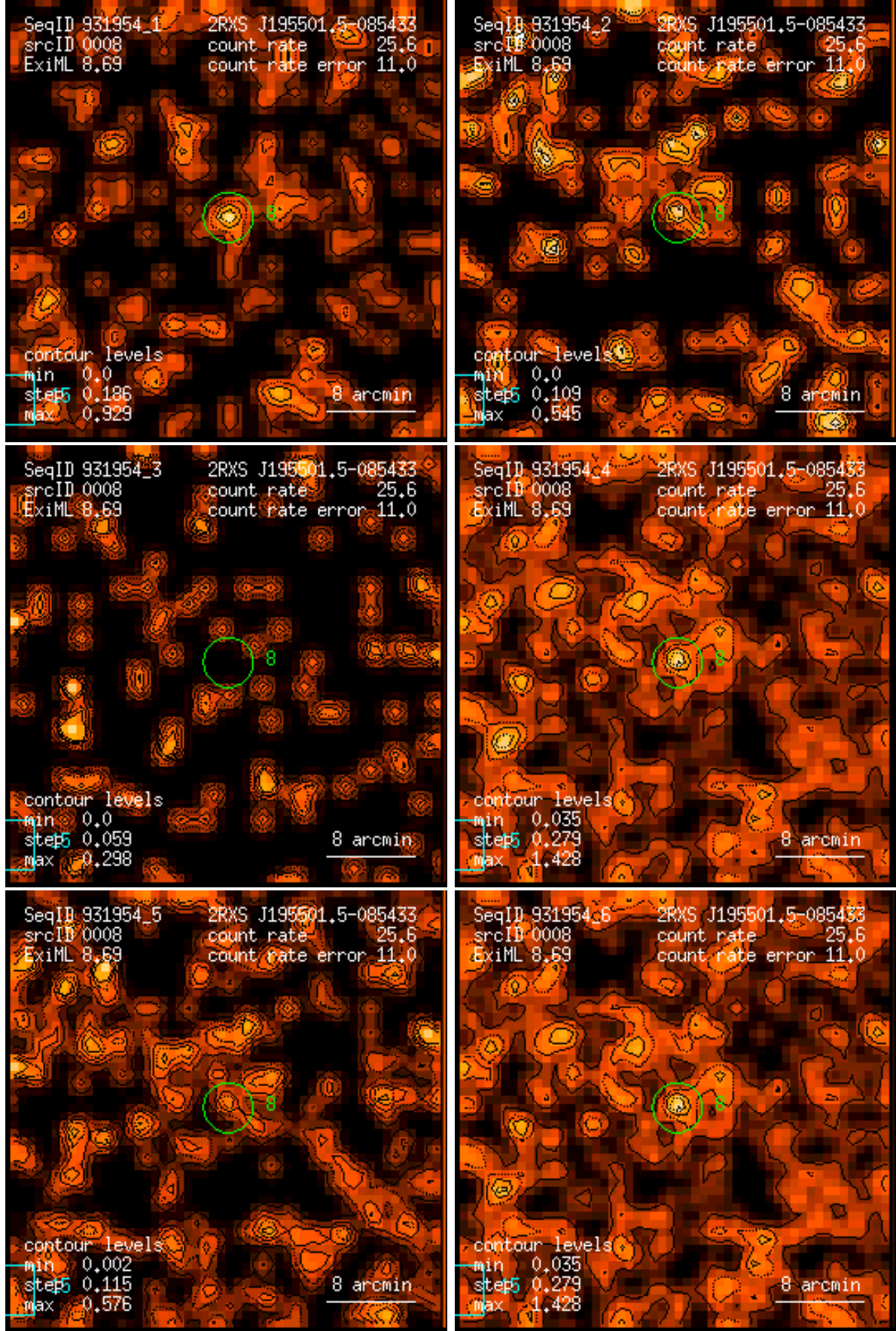
Figure 8: RASS 931954: detection 0008: band rate images, Gaussian filter: (1) PSPC channels 11 – 41, (2) 52 – 90, (3) 91 – 201, (4) 11 – 235, (5) 52 – 201, (6) 11 – 201. Broad band rates in counts/ks. Band rate contour levels in counts/ks/arcmin 2 .
