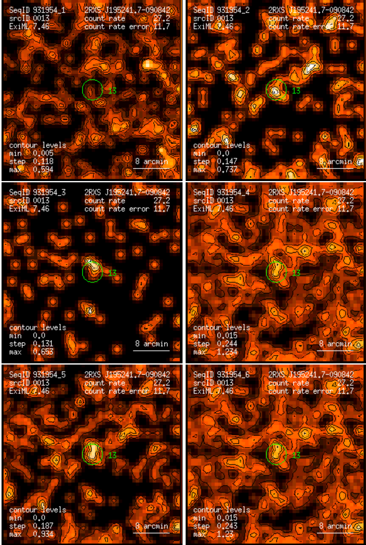
Figure 13: RASS 931954: detection 0013: band rate images, Gaussian filter: (1) PSPC channels 11 – 41, (2) 52 – 90, (3) 91 – 201, (4) 11 – 235, (5) 52 – 201, (6) 11 – 201. Broad band rates in counts/ks. Band rate contour levels in counts/ks/arcmin 2 .
