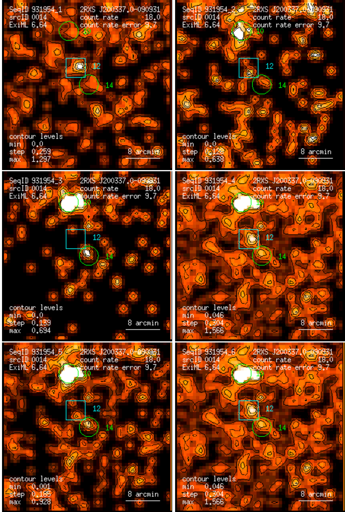
Figure 14: RASS 931954: detection 0014: band rate images, Gaussian filter: (1) PSPC channels 11 – 41, (2) 52 – 90, (3) 91 – 201, (4) 11 – 235, (5) 52 – 201, (6) 11 – 201. Broad band rates in counts/ks. Band rate contour levels in counts/ks/arcmin 2 .
