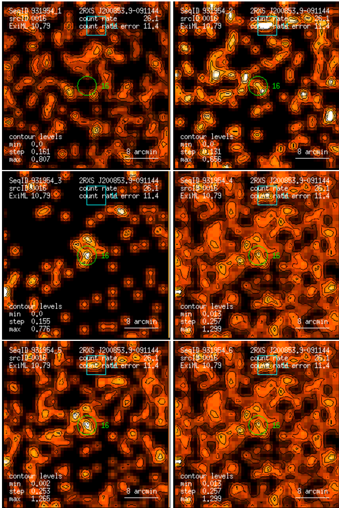
Figure 16: RASS 931954: detection 0016: band rate images, Gaussian filter: (1) PSPC channels 11 – 41, (2) 52 – 90, (3) 91 – 201, (4) 11 – 235, (5) 52 – 201, (6) 11 – 201. Broad band rates in counts/ks. Band rate contour levels in counts/ks/arcmin 2 .
