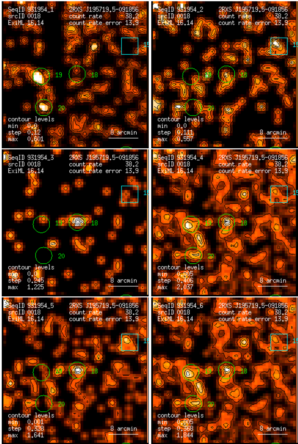
Figure 18: RASS 931954: detection 0018: band rate images, Gaussian filter: (1) PSPC channels 11 – 41, (2) 52 – 90, (3) 91 – 201, (4) 11 – 235, (5) 52 – 201, (6) 11 – 201. Broad band rates in counts/ks. Band rate contour levels in counts/ks/arcmin 2 .
