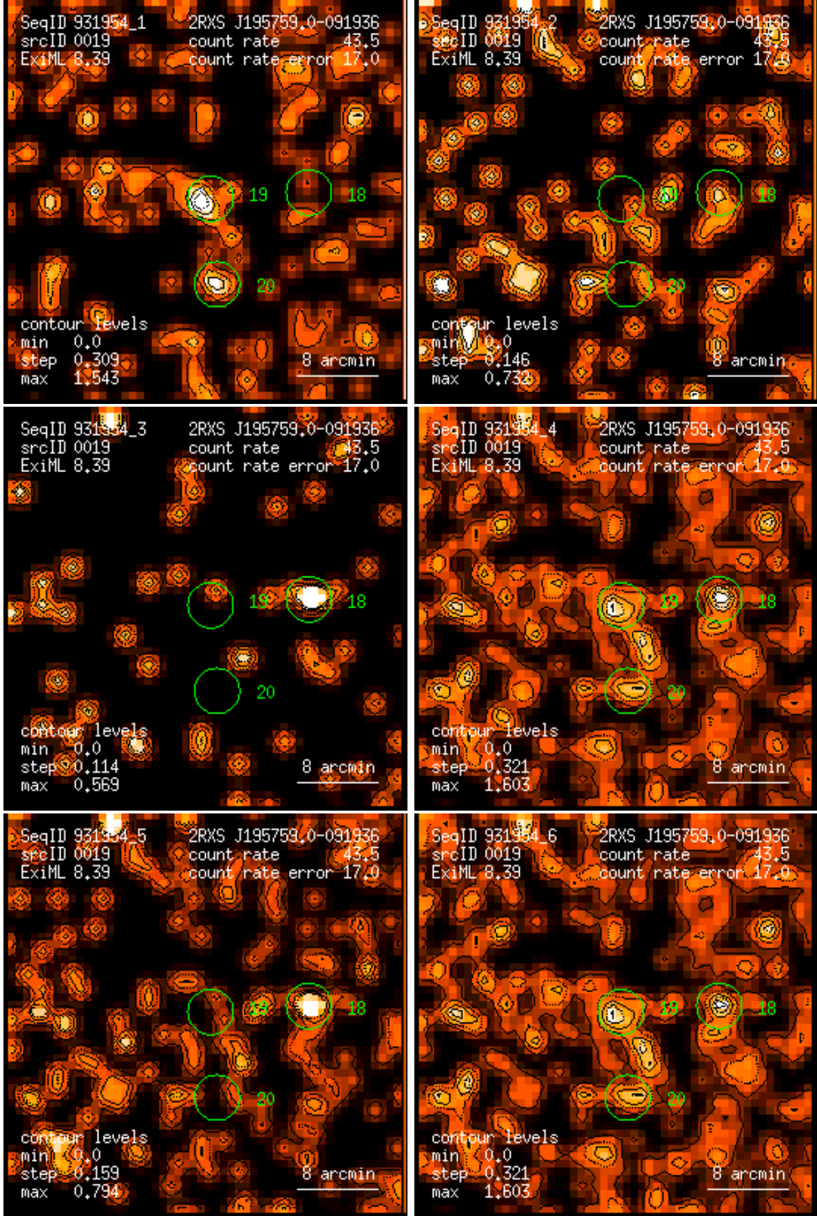
Figure 19: RASS 931954: detection 0019: band rate images, Gaussian filter: (1) PSPC channels 11 – 41, (2) 52 – 90, (3) 91 – 201, (4) 11 – 235, (5) 52 – 201, (6) 11 – 201. Broad band rates in counts/ks. Band rate contour levels in counts/ks/arcmin 2 .
