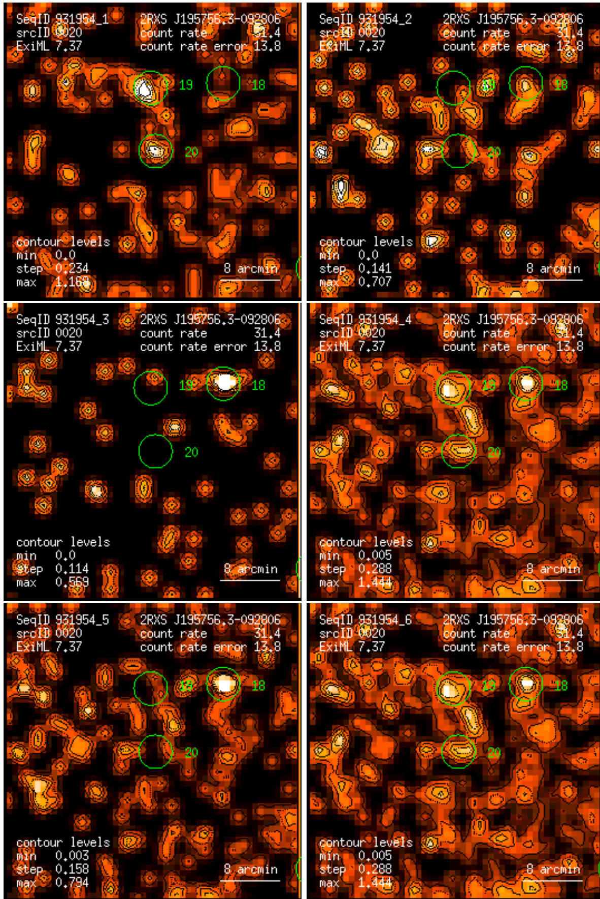
Figure 20: RASS 931954: detection 0020: band rate images, Gaussian filter: (1) PSPC channels 11 – 41, (2) 52 – 90, (3) 91 – 201, (4) 11 – 235, (5) 52 – 201, (6) 11 – 201. Broad band rates in counts/ks. Band rate contour levels in counts/ks/arcmin 2 .
