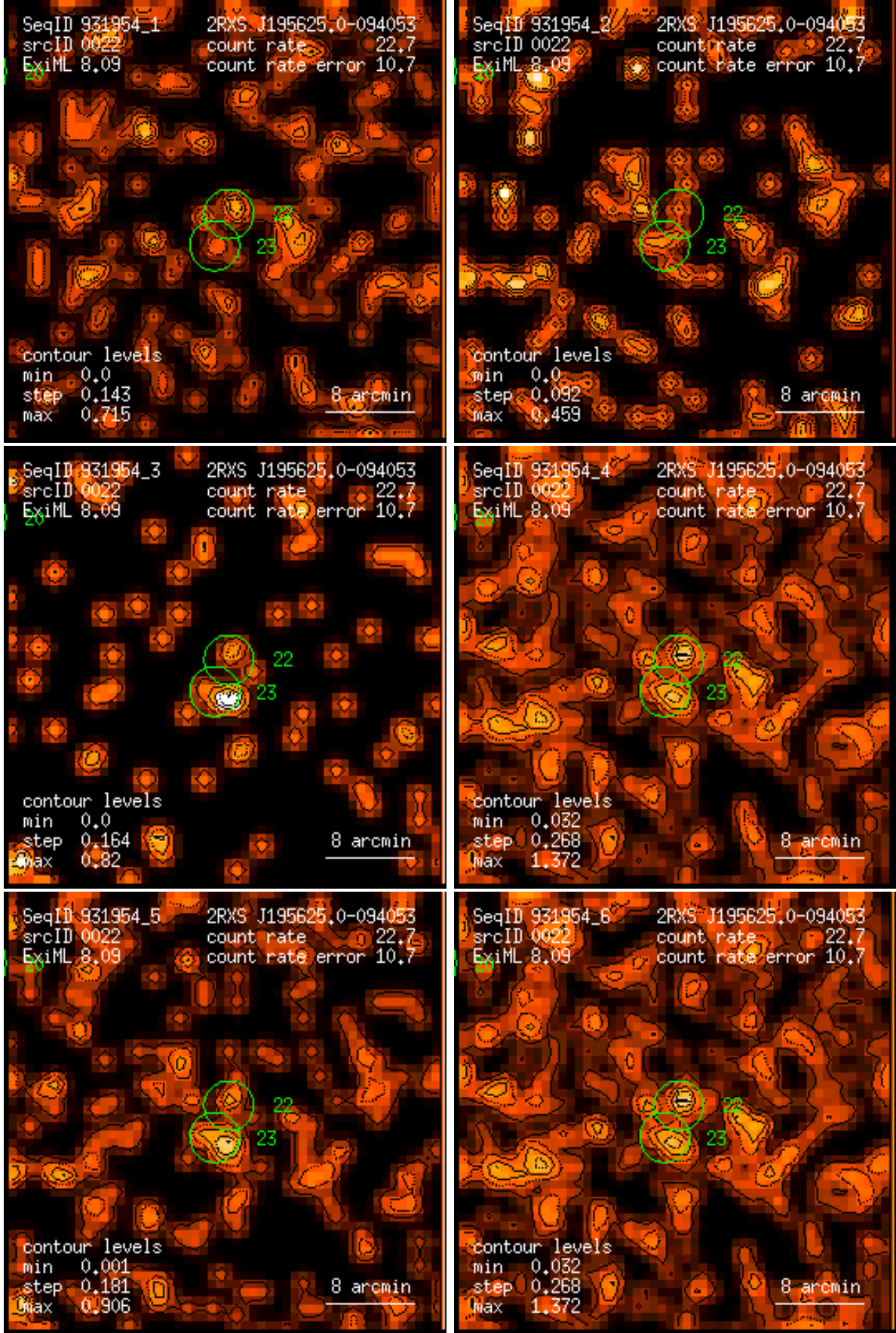
Figure 22: RASS 931954: detection 0022: band rate images, Gaussian filter: (1) PSPC channels 11 – 41, (2) 52 – 90, (3) 91 – 201, (4) 11 – 235, (5) 52 – 201, (6) 11 – 201. Broad band rates in counts/ks. Band rate contour levels in counts/ks/arcmin 2 .
