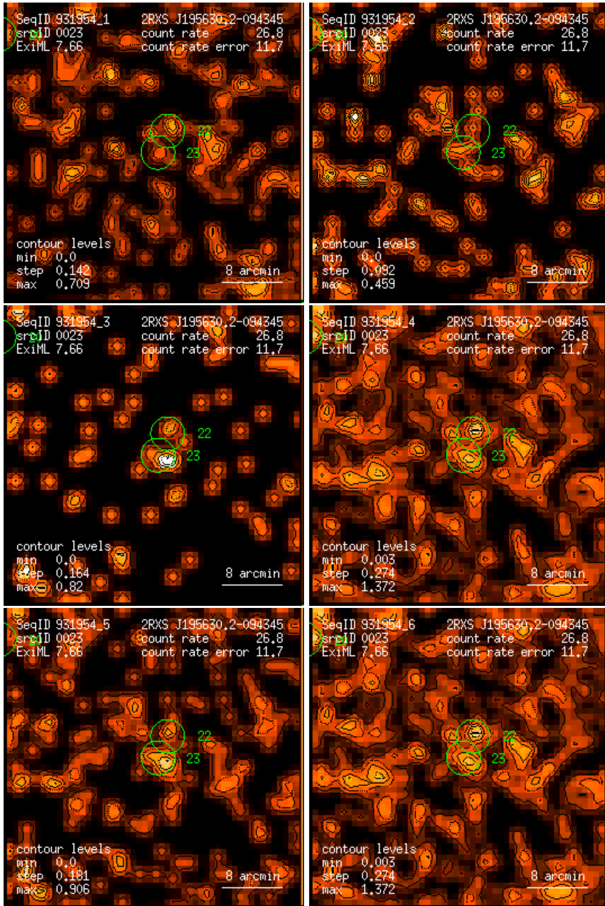
Figure 23: RASS 931954: detection 0023: band rate images, Gaussian filter: (1) PSPC channels 11 – 41, (2) 52 – 90, (3) 91 – 201, (4) 11 – 235, (5) 52 – 201, (6) 11 – 201. Broad band rates in counts/ks. Band rate contour levels in counts/ks/arcmin 2 .
