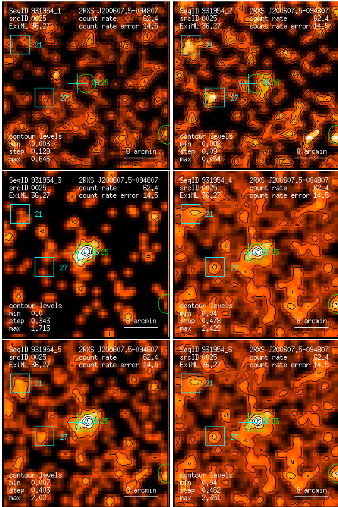
Figure 25: RASS 931954: detection 0025: band rate images, Gaussian filter: (1) PSPC channels 11 – 41, (2) 52 – 90, (3) 91 – 201, (4) 11 – 235, (5) 52 – 201, (6) 11 – 201. Broad band rates in counts/ks. Band rate contour levels in counts/ks/arcmin 2 .
