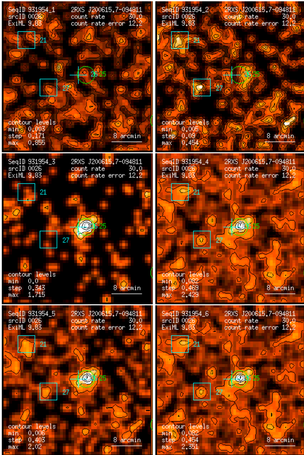
Figure 26: RASS 931954: detection 0026: band rate images, Gaussian filter: (1) PSPC channels 11 – 41, (2) 52 – 90, (3) 91 – 201, (4) 11 – 235, (5) 52 – 201, (6) 11 – 201. Broad band rates in counts/ks. Band rate contour levels in counts/ks/arcmin 2 .
