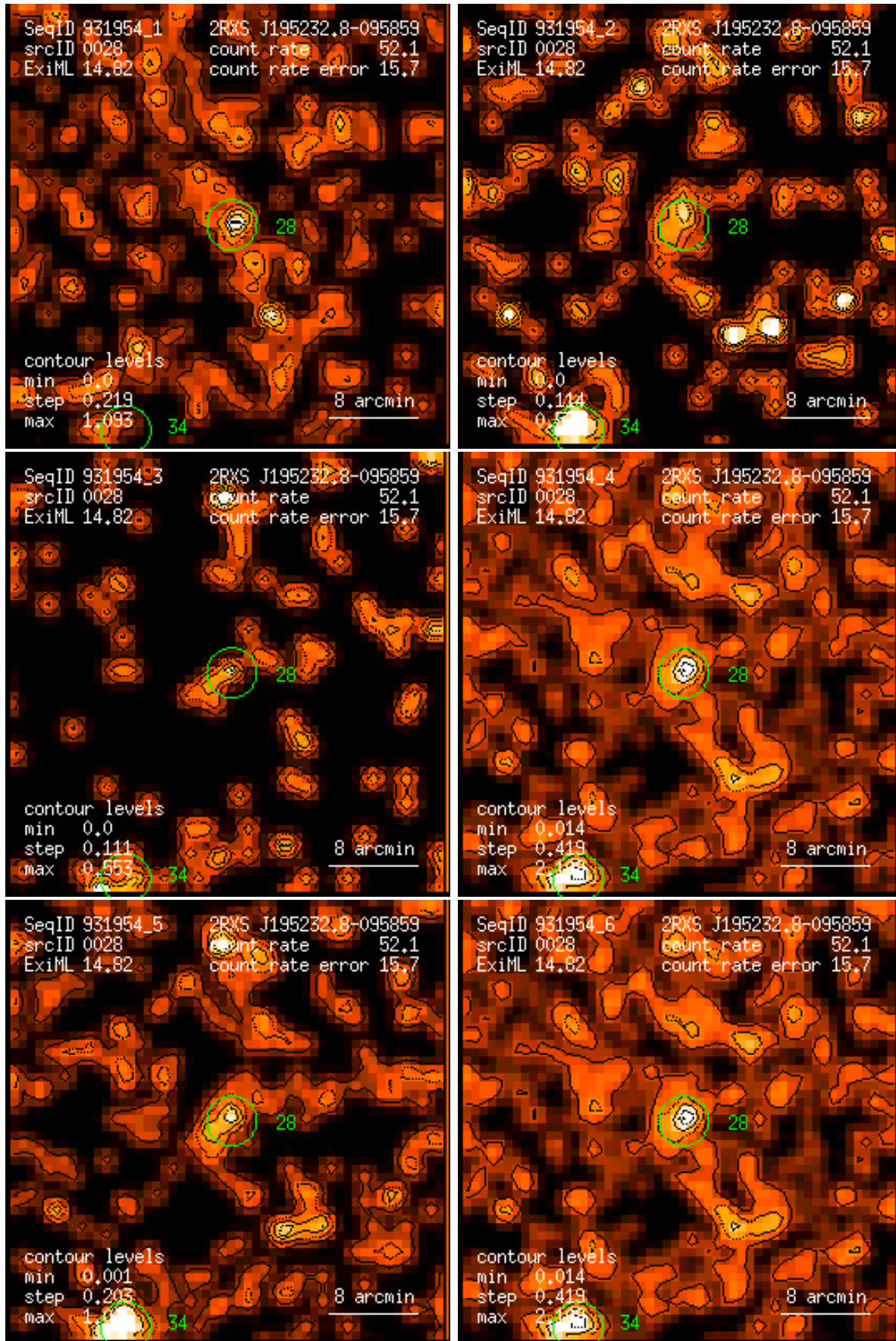
Figure 28: RASS 931954: detection 0028: band rate images, Gaussian filter: (1) PSPC channels 11 – 41, (2) 52 – 90, (3) 91 – 201, (4) 11 – 235, (5) 52 – 201, (6) 11 – 201. Broad band rates in counts/ks. Band rate contour levels in counts/ks/arcmin 2 .
