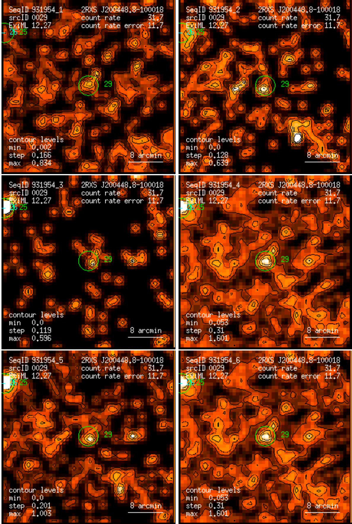
Figure 29: RASS 931954: detection 0029: band rate images, Gaussian filter: (1) PSPC channels 11 – 41, (2) 52 – 90, (3) 91 – 201, (4) 11 – 235, (5) 52 – 201, (6) 11 – 201. Broad band rates in counts/ks. Band rate contour levels in counts/ks/arcmin 2 .
