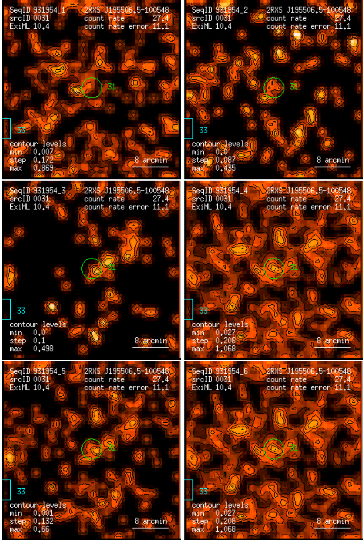
Figure 31: RASS 931954: detection 0031: band rate images, Gaussian filter: (1) PSPC channels 11 – 41, (2) 52 – 90, (3) 91 – 201, (4) 11 – 235, (5) 52 – 201, (6) 11 – 201. Broad band rates in counts/ks. Band rate contour levels in counts/ks/arcmin 2 .
