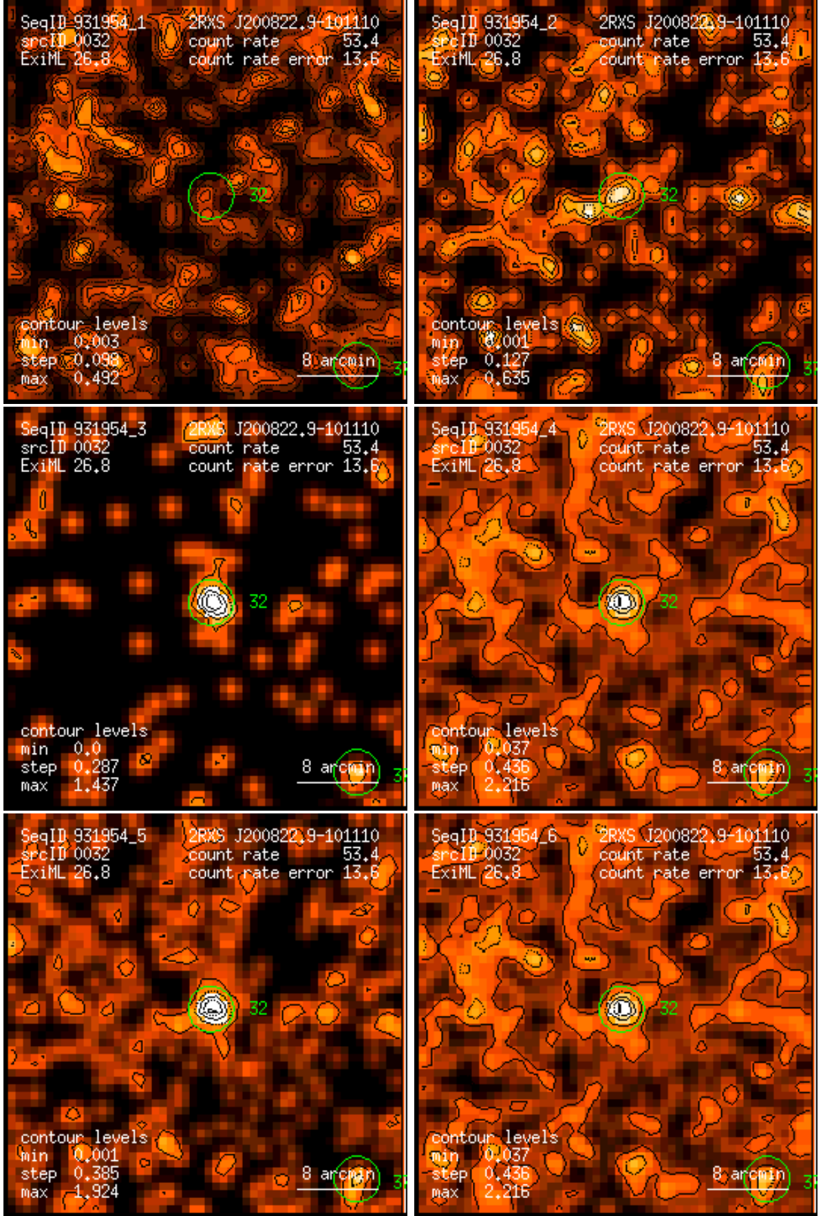
Figure 32: RASS 931954: detection 0032: band rate images, Gaussian filter: (1) PSPC channels 11 – 41, (2) 52 – 90, (3) 91 – 201, (4) 11 – 235, (5) 52 – 201, (6) 11 – 201. Broad band rates in counts/ks. Band rate contour levels in counts/ks/arcmin 2 .
