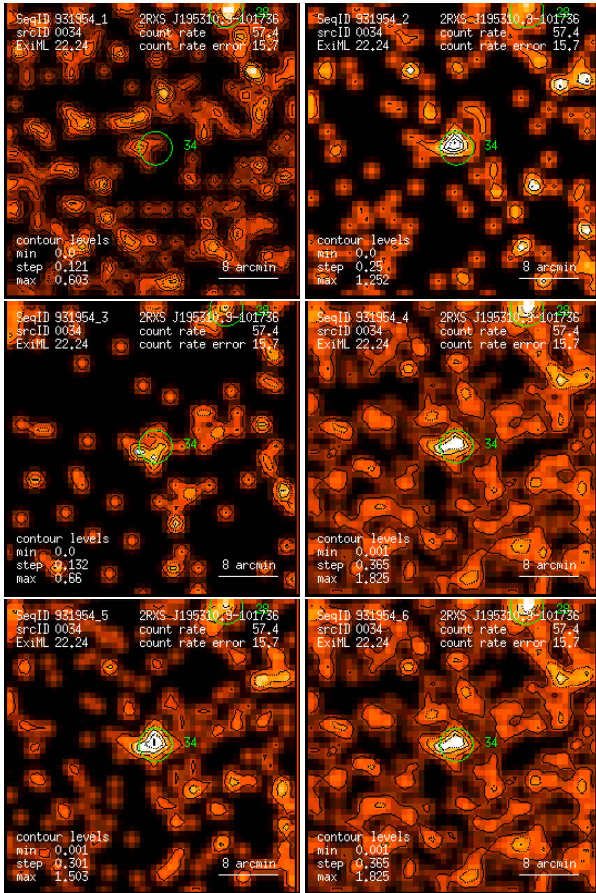
Figure 34: RASS 931954: detection 0034: band rate images, Gaussian filter: (1) PSPC channels 11 – 41, (2) 52 – 90, (3) 91 – 201, (4) 11 – 235, (5) 52 – 201, (6) 11 – 201. Broad band rates in counts/ks. Band rate contour levels in counts/ks/arcmin 2 .
