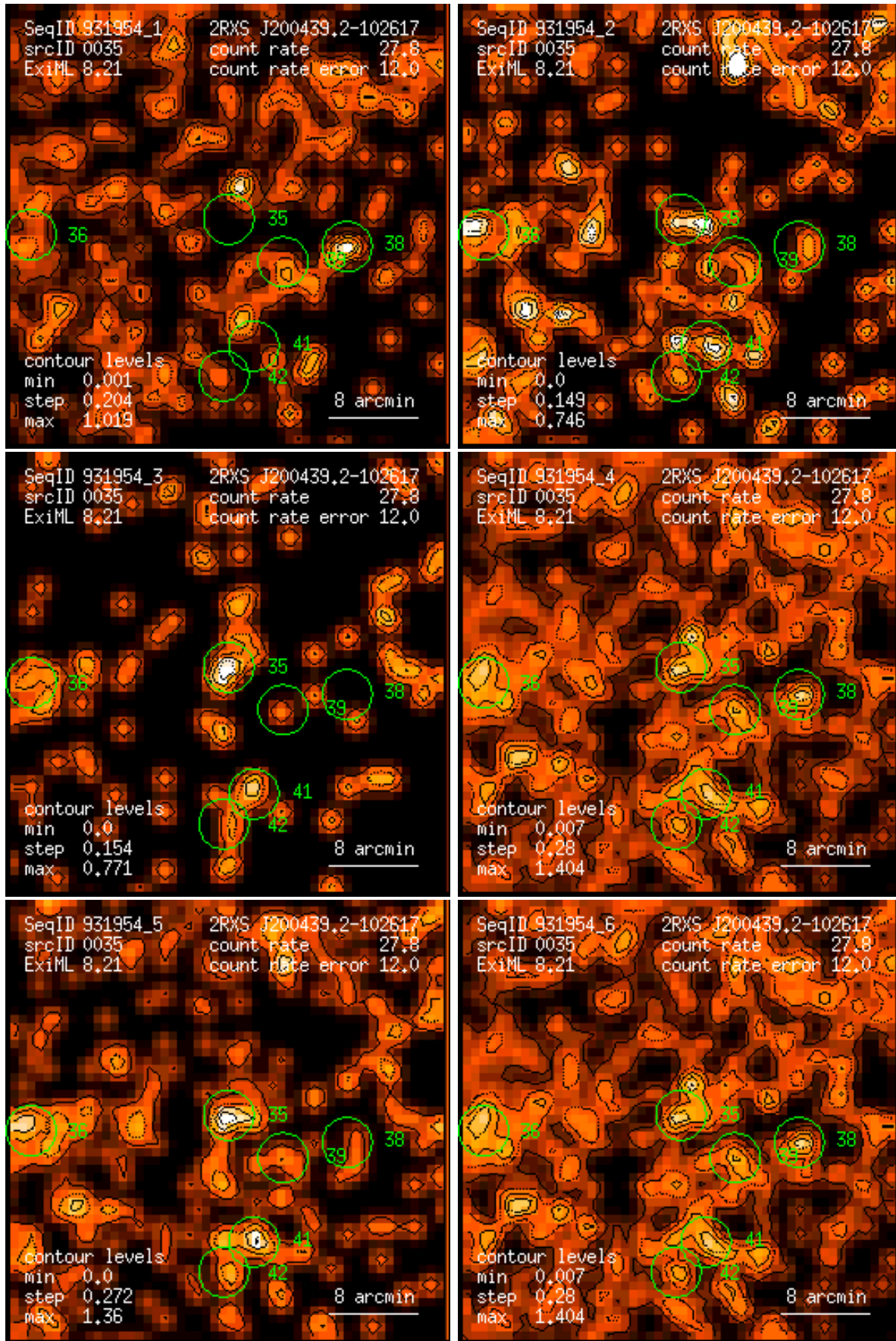
Figure 35: RASS 931954: detection 0035: band rate images, Gaussian filter: (1) PSPC channels 11 – 41, (2) 52 – 90, (3) 91 – 201, (4) 11 – 235, (5) 52 – 201, (6) 11 – 201. Broad band rates in counts/ks. Band rate contour levels in counts/ks/arcmin 2 .
