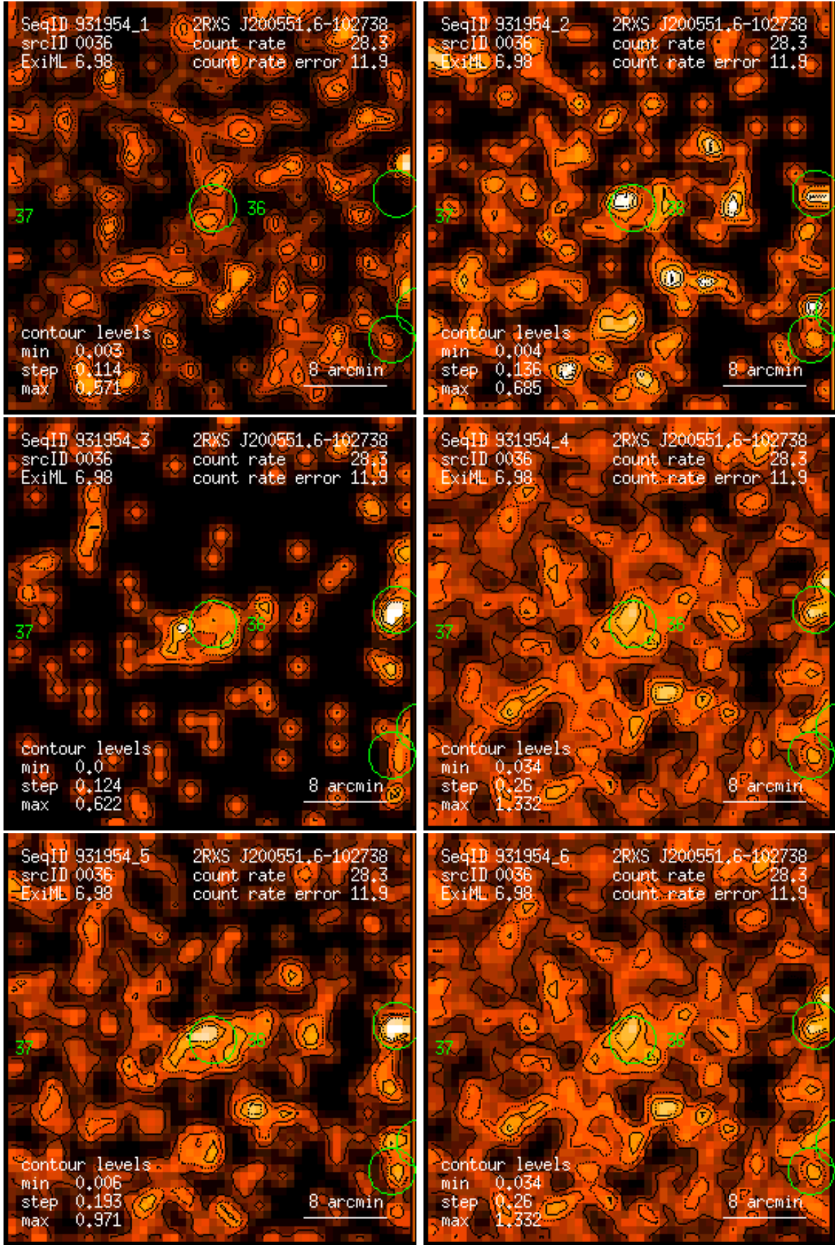
Figure 36: RASS 931954: detection 0036: band rate images, Gaussian filter: (1) PSPC channels 11 – 41, (2) 52 – 90, (3) 91 – 201, (4) 11 – 235, (5) 52 – 201, (6) 11 – 201. Broad band rates in counts/ks. Band rate contour levels in counts/ks/arcmin 2 .
