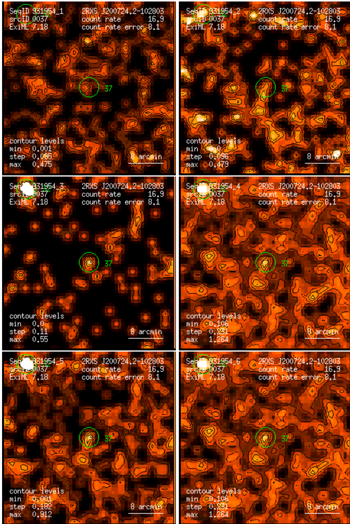
Figure 37: RASS 931954: detection 0037: band rate images, Gaussian filter: (1) PSPC channels 11 – 41, (2) 52 – 90, (3) 91 – 201, (4) 11 – 235, (5) 52 – 201, (6) 11 – 201. Broad band rates in counts/ks. Band rate contour levels in counts/ks/arcmin 2 .
