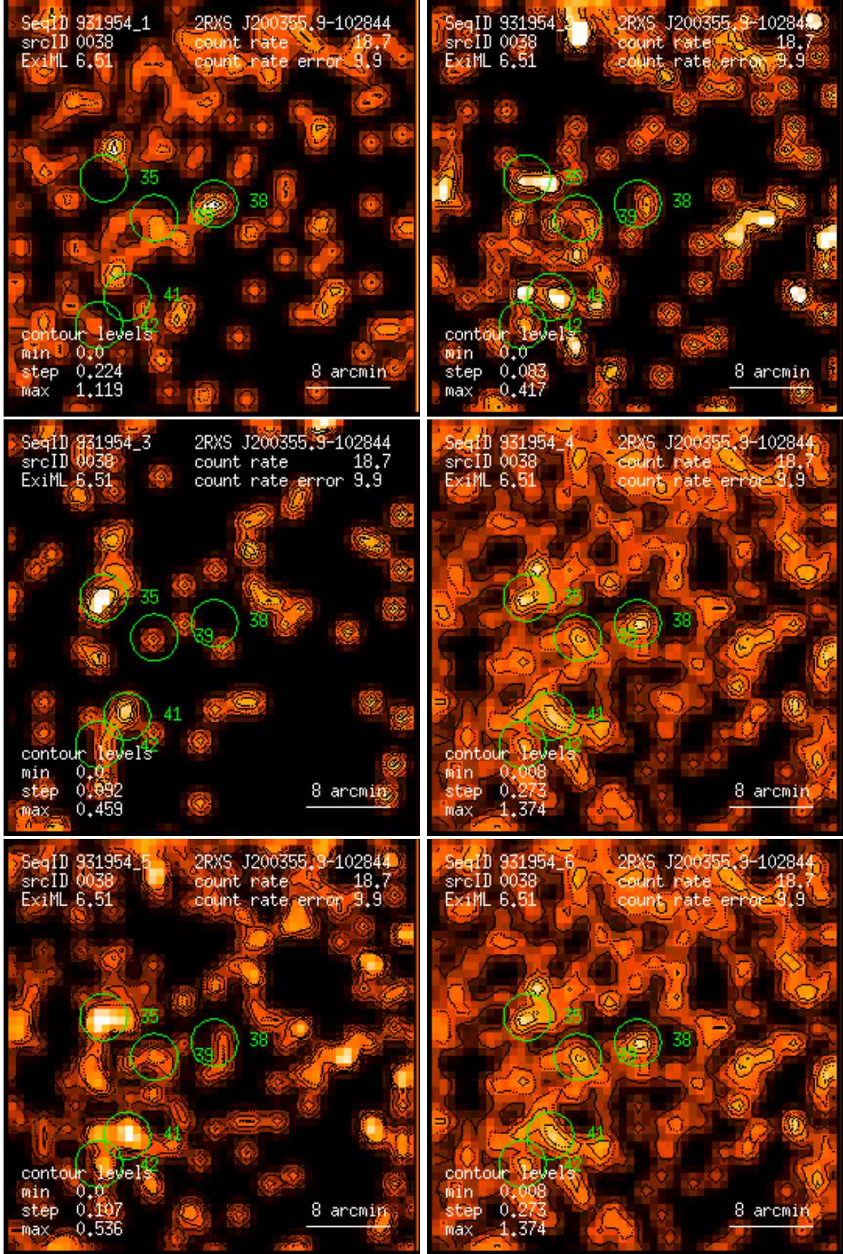
Figure 38: RASS 931954: detection 0038: band rate images, Gaussian filter: (1) PSPC channels 11 – 41, (2) 52 – 90, (3) 91 – 201, (4) 11 – 235, (5) 52 – 201, (6) 11 – 201. Broad band rates in counts/ks. Band rate contour levels in counts/ks/arcmin 2 .
