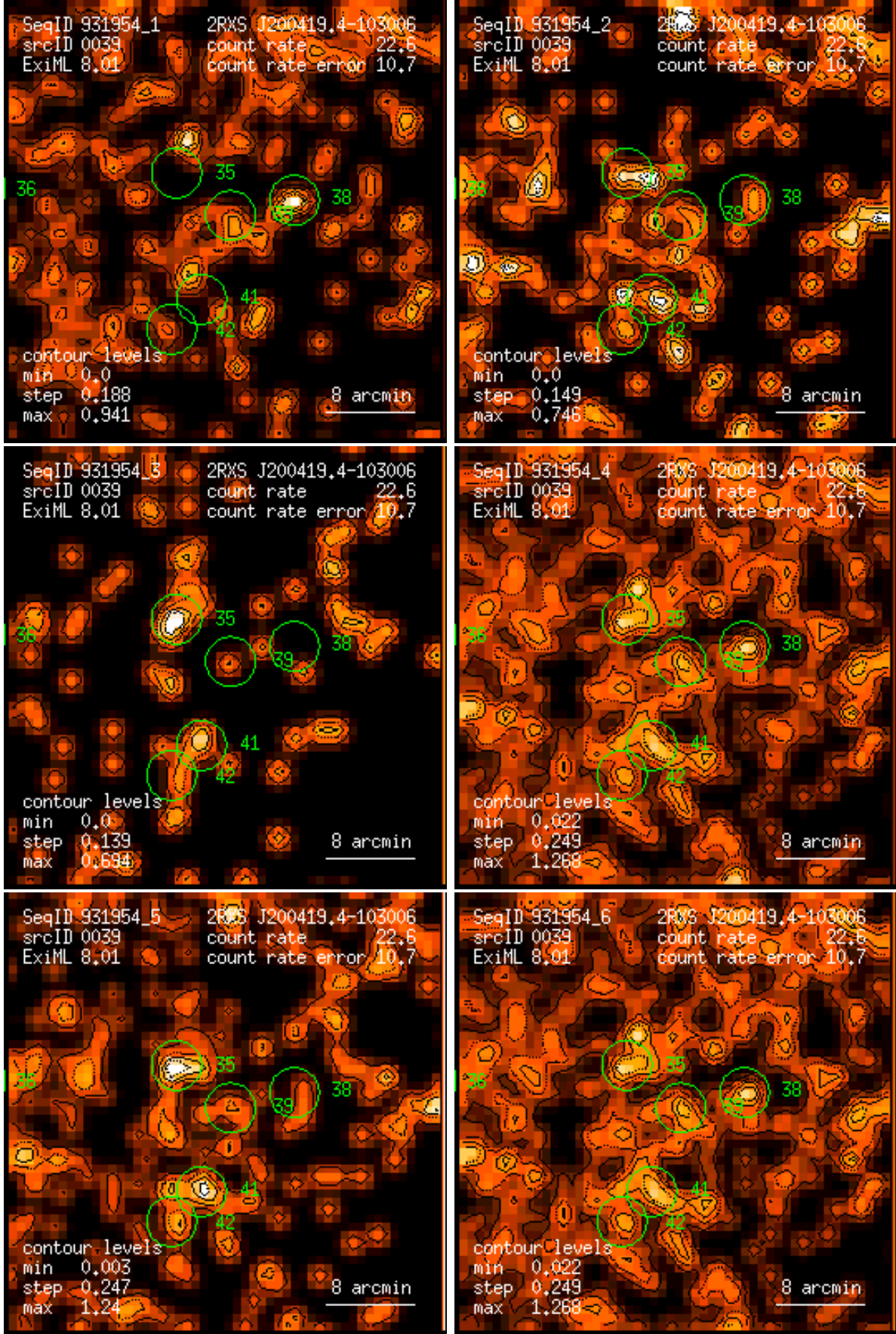
Figure 39: RASS 931954: detection 0039: band rate images, Gaussian filter: (1) PSPC channels 11 – 41, (2) 52 – 90, (3) 91 – 201, (4) 11 – 235, (5) 52 – 201, (6) 11 – 201. Broad band rates in counts/ks. Band rate contour levels in counts/ks/arcmin 2 .
