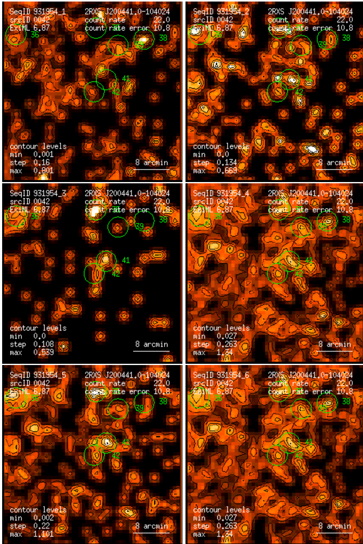
Figure 42: RASS 931954: detection 0042: band rate images, Gaussian filter: (1) PSPC channels 11 – 41, (2) 52 – 90, (3) 91 – 201, (4) 11 – 235, (5) 52 – 201, (6) 11 – 201. Broad band rates in counts/ks. Band rate contour levels in counts/ks/arcmin 2 .
