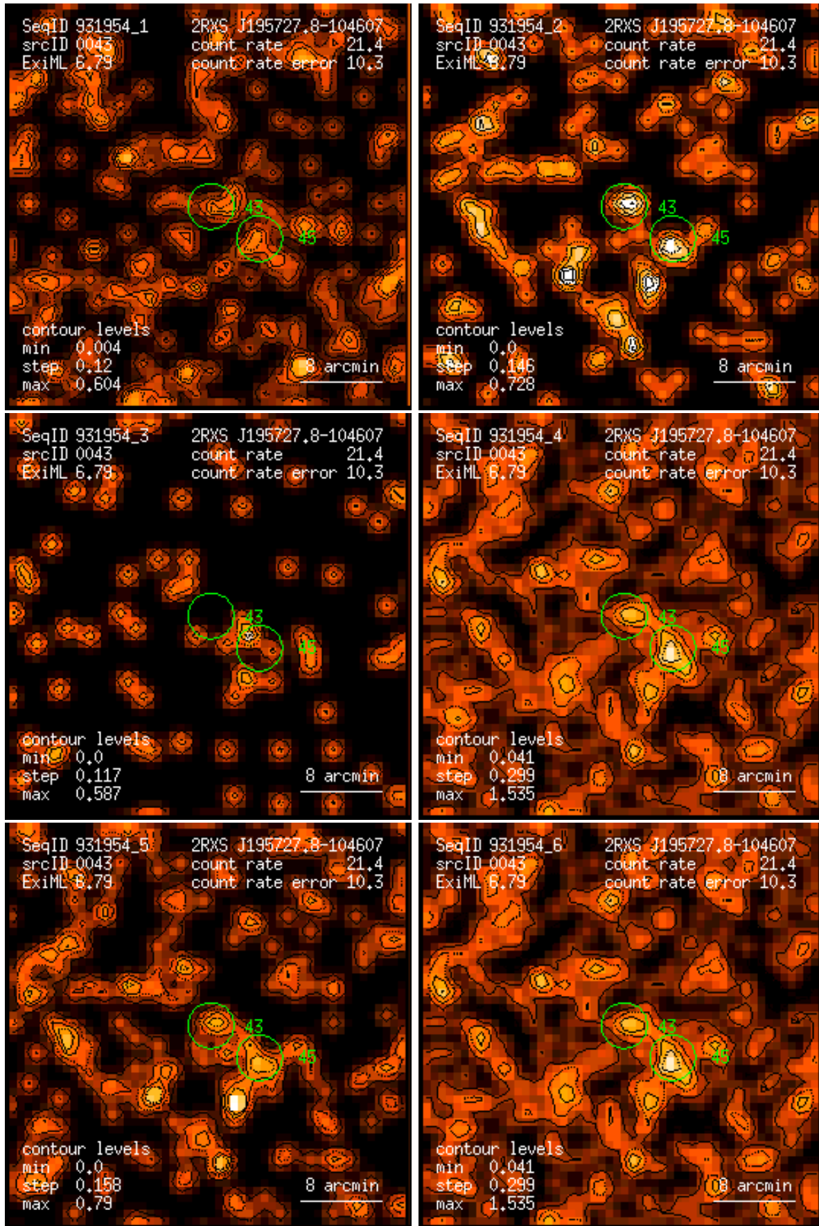
Figure 43: RASS 931954: detection 0043: band rate images, Gaussian filter: (1) PSPC channels 11 – 41, (2) 52 – 90, (3) 91 – 201, (4) 11 – 235, (5) 52 – 201, (6) 11 – 201. Broad band rates in counts/ks. Band rate contour levels in counts/ks/arcmin 2 .
