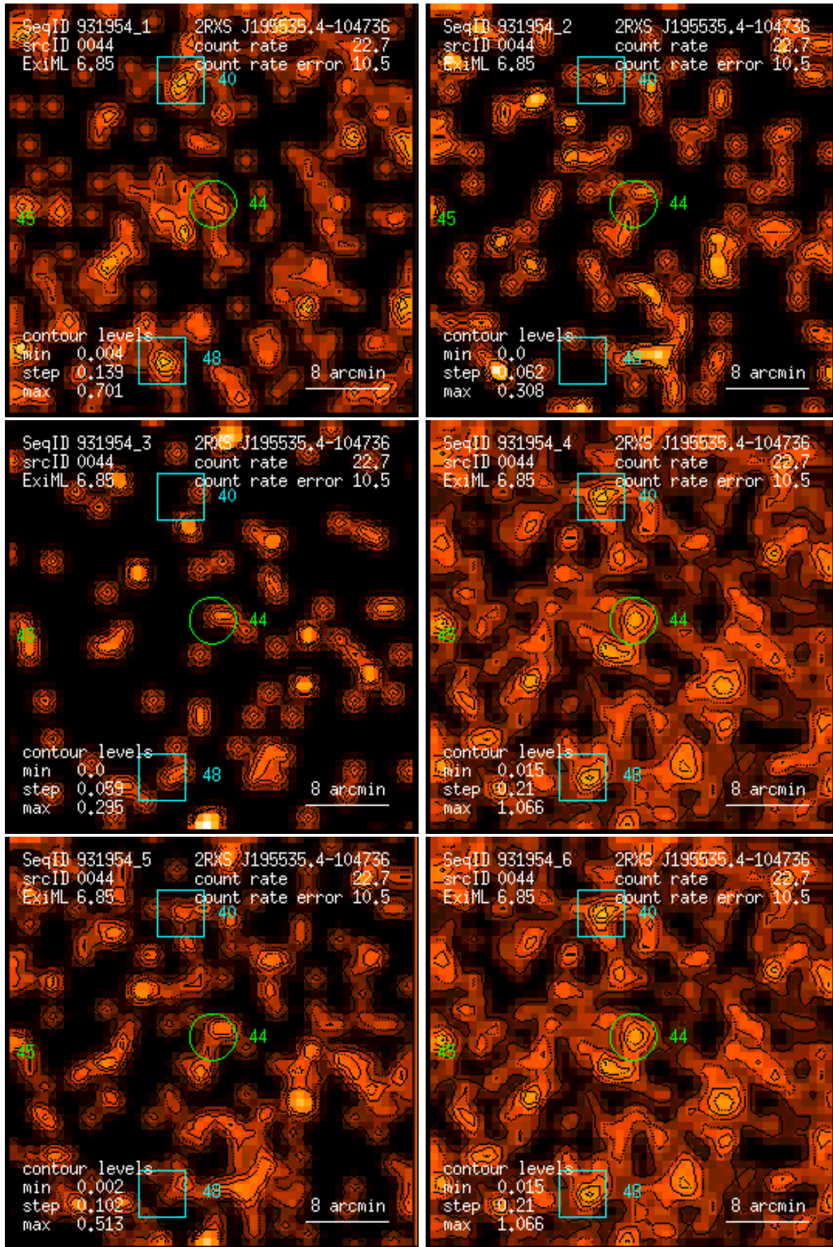
Figure 44: RASS 931954: detection 0044: band rate images, Gaussian filter: (1) PSPC channels 11 – 41, (2) 52 – 90, (3) 91 – 201, (4) 11 – 235, (5) 52 – 201, (6) 11 – 201. Broad band rates in counts/ks. Band rate contour levels in counts/ks/arcmin 2 .
