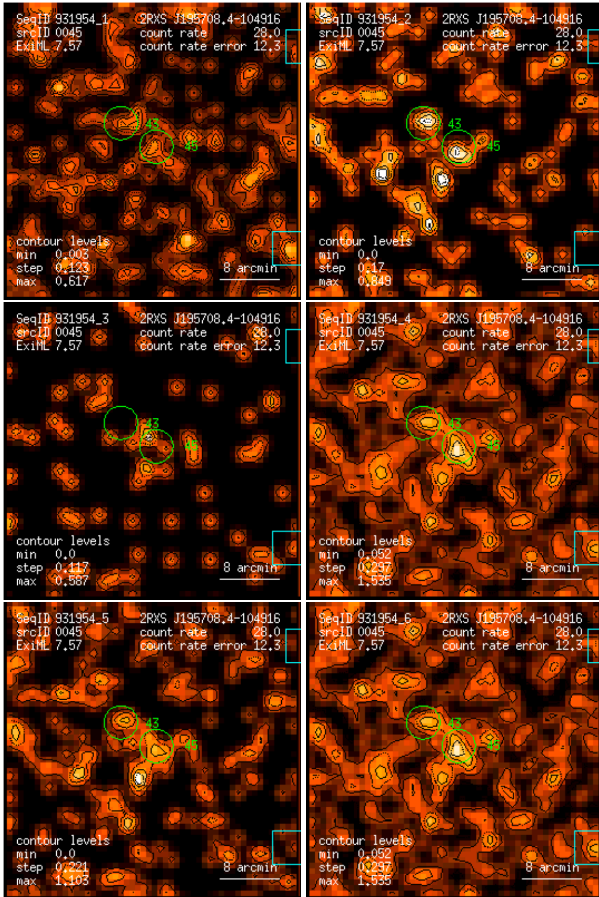
Figure 45: RASS 931954: detection 0045: band rate images, Gaussian filter: (1) PSPC channels 11 – 41, (2) 52 – 90, (3) 91 – 201, (4) 11 – 235, (5) 52 – 201, (6) 11 – 201. Broad band rates in counts/ks. Band rate contour levels in counts/ks/arcmin 2 .
