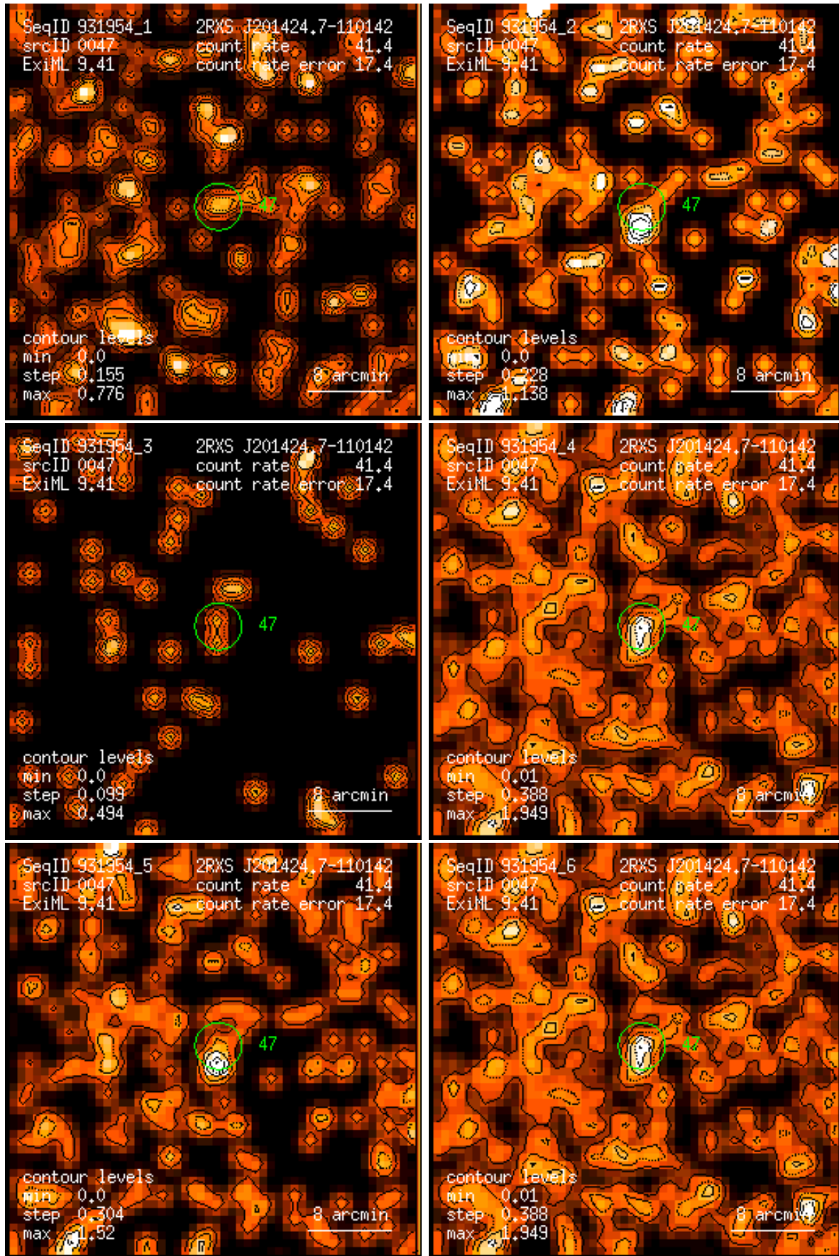
Figure 47: RASS 931954: detection 0047: band rate images, Gaussian filter: (1) PSPC channels 11 – 41, (2) 52 – 90, (3) 91 – 201, (4) 11 – 235, (5) 52 – 201, (6) 11 – 201. Broad band rates in counts/ks. Band rate contour levels in counts/ks/arcmin 2 .
