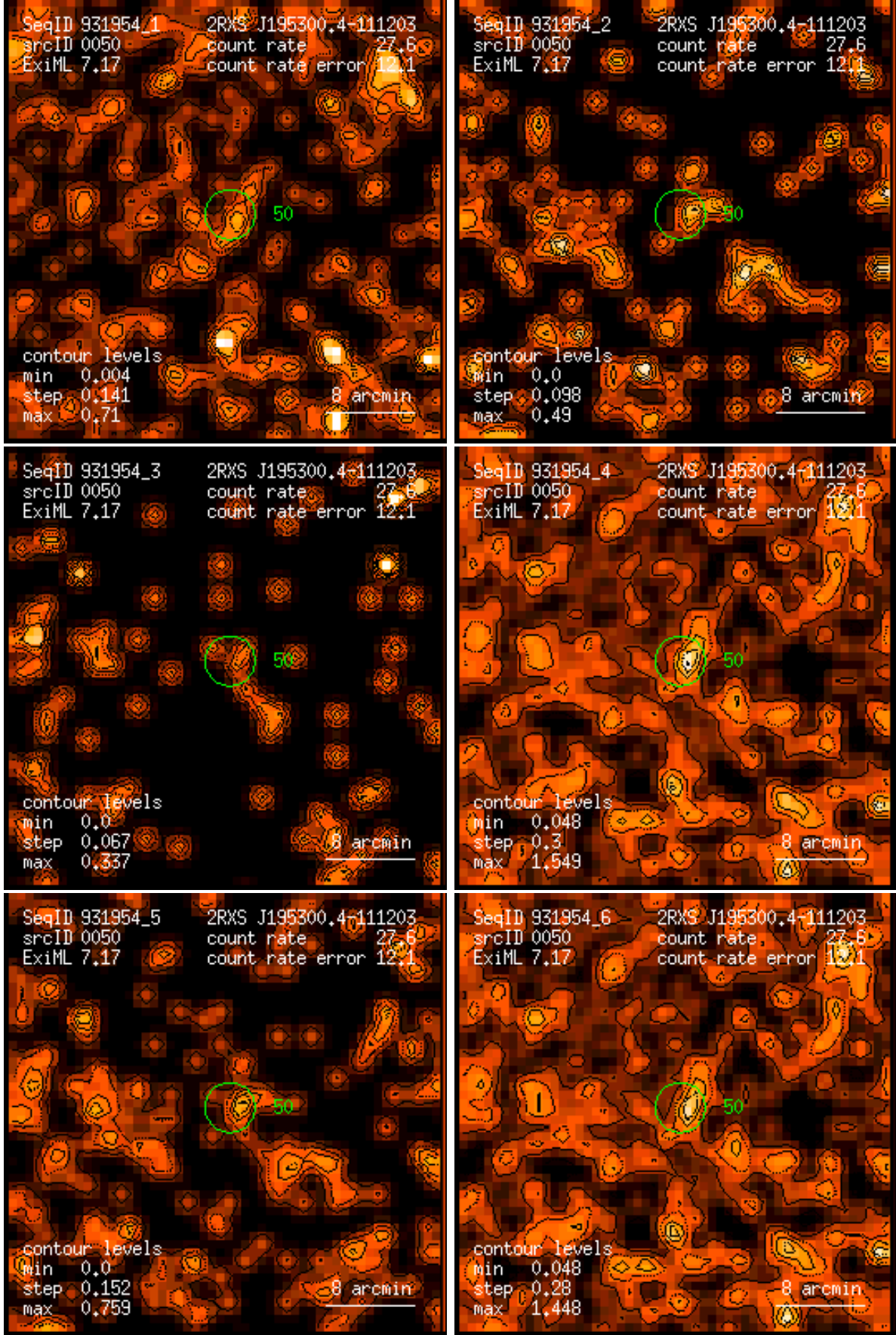
Figure 50: RASS 931954: detection 0050: band rate images, Gaussian filter: (1) PSPC channels 11 – 41, (2) 52 – 90, (3) 91 – 201, (4) 11 – 235, (5) 52 – 201, (6) 11 – 201. Broad band rates in counts/ks. Band rate contour levels in counts/ks/arcmin 2 .
