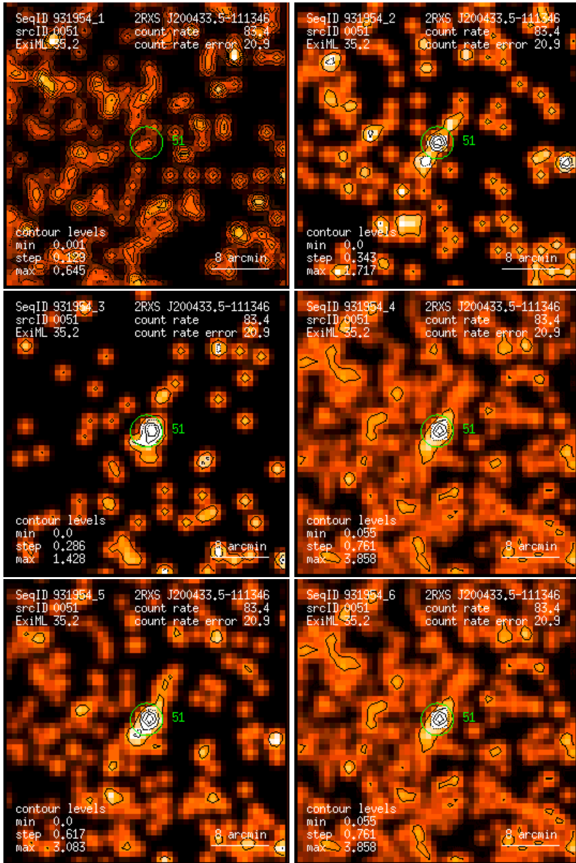
Figure 51: RASS 931954: detection 0051: band rate images, Gaussian filter: (1) PSPC channels 11 – 41, (2) 52 – 90, (3) 91 – 201, (4) 11 – 235, (5) 52 – 201, (6) 11 – 201. Broad band rates in counts/ks. Band rate contour levels in counts/ks/arcmin 2 .
