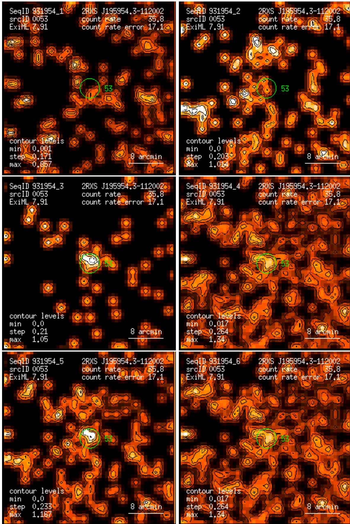
Figure 53: RASS 931954: detection 0053: band rate images, Gaussian filter: (1) PSPC channels 11 – 41, (2) 52 – 90, (3) 91 – 201, (4) 11 – 235, (5) 52 – 201, (6) 11 – 201. Broad band rates in counts/ks. Band rate contour levels in counts/ks/arcmin 2 .
