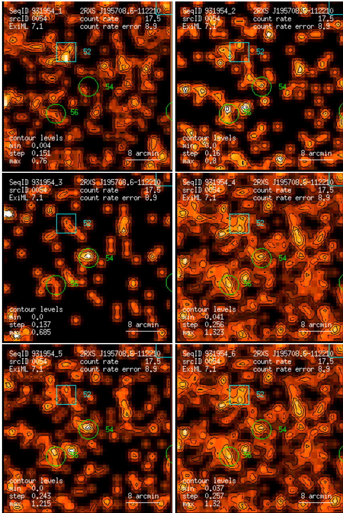
Figure 54: RASS 931954: detection 0054: band rate images, Gaussian filter: (1) PSPC channels 11 – 41, (2) 52 – 90, (3) 91 – 201, (4) 11 – 235, (5) 52 – 201, (6) 11 – 201. Broad band rates in counts/ks. Band rate contour levels in counts/ks/arcmin 2 .
