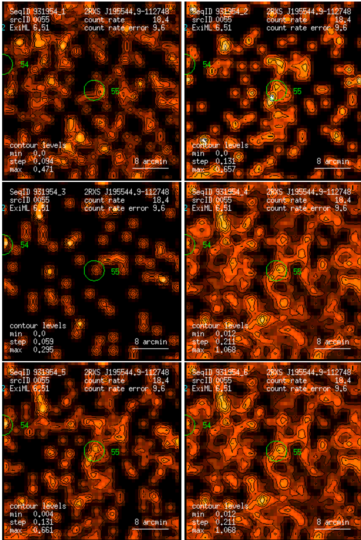
Figure 55: RASS 931954: detection 0055: band rate images, Gaussian filter: (1) PSPC channels 11 – 41, (2) 52 – 90, (3) 91 – 201, (4) 11 – 235, (5) 52 – 201, (6) 11 – 201. Broad band rates in counts/ks. Band rate contour levels in counts/ks/arcmin 2 .
