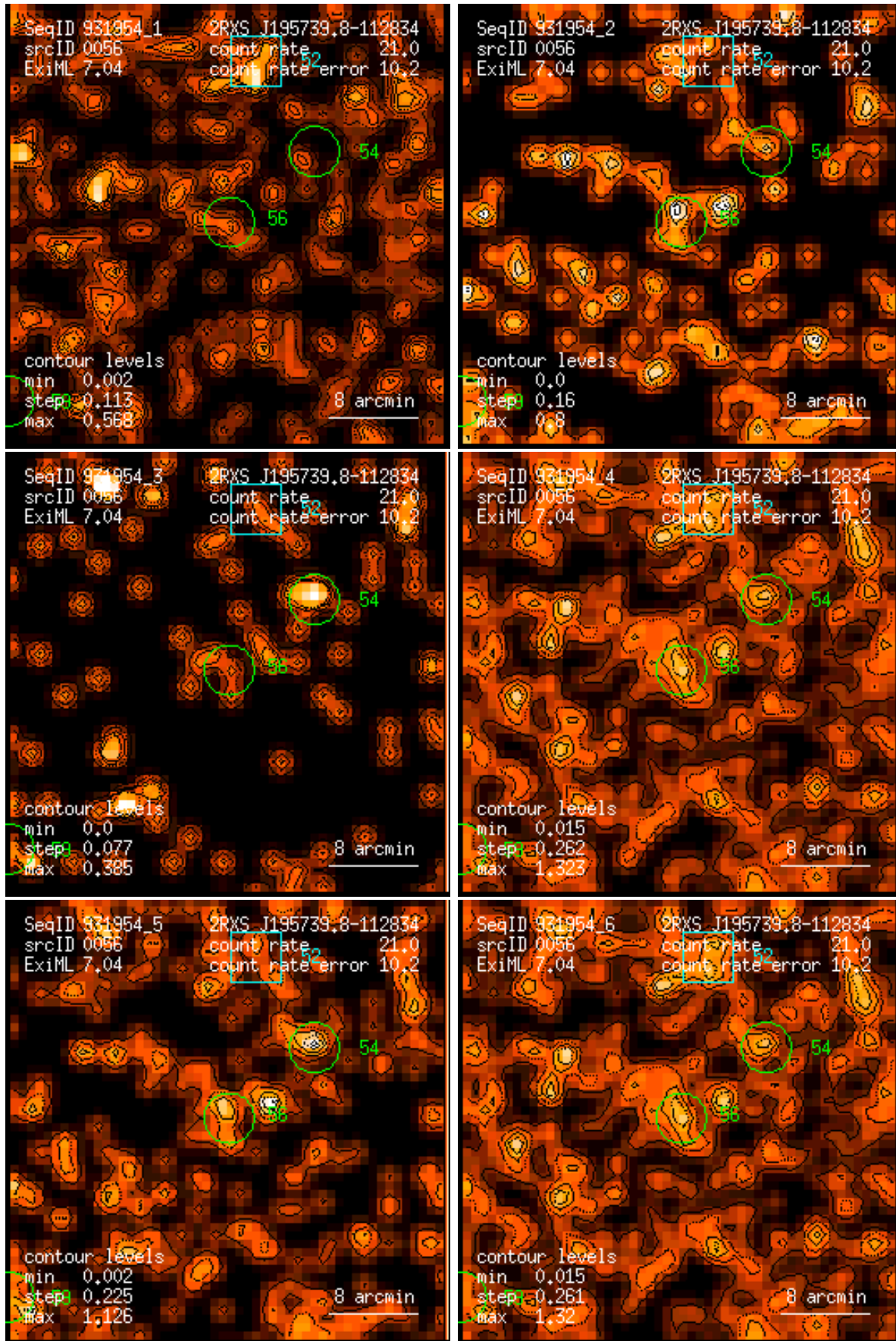
Figure 56: RASS 931954: detection 0056: band rate images, Gaussian filter: (1) PSPC channels 11 – 41, (2) 52 – 90, (3) 91 – 201, (4) 11 – 235, (5) 52 – 201, (6) 11 – 201. Broad band rates in counts/ks. Band rate contour levels in counts/ks/arcmin 2 .
