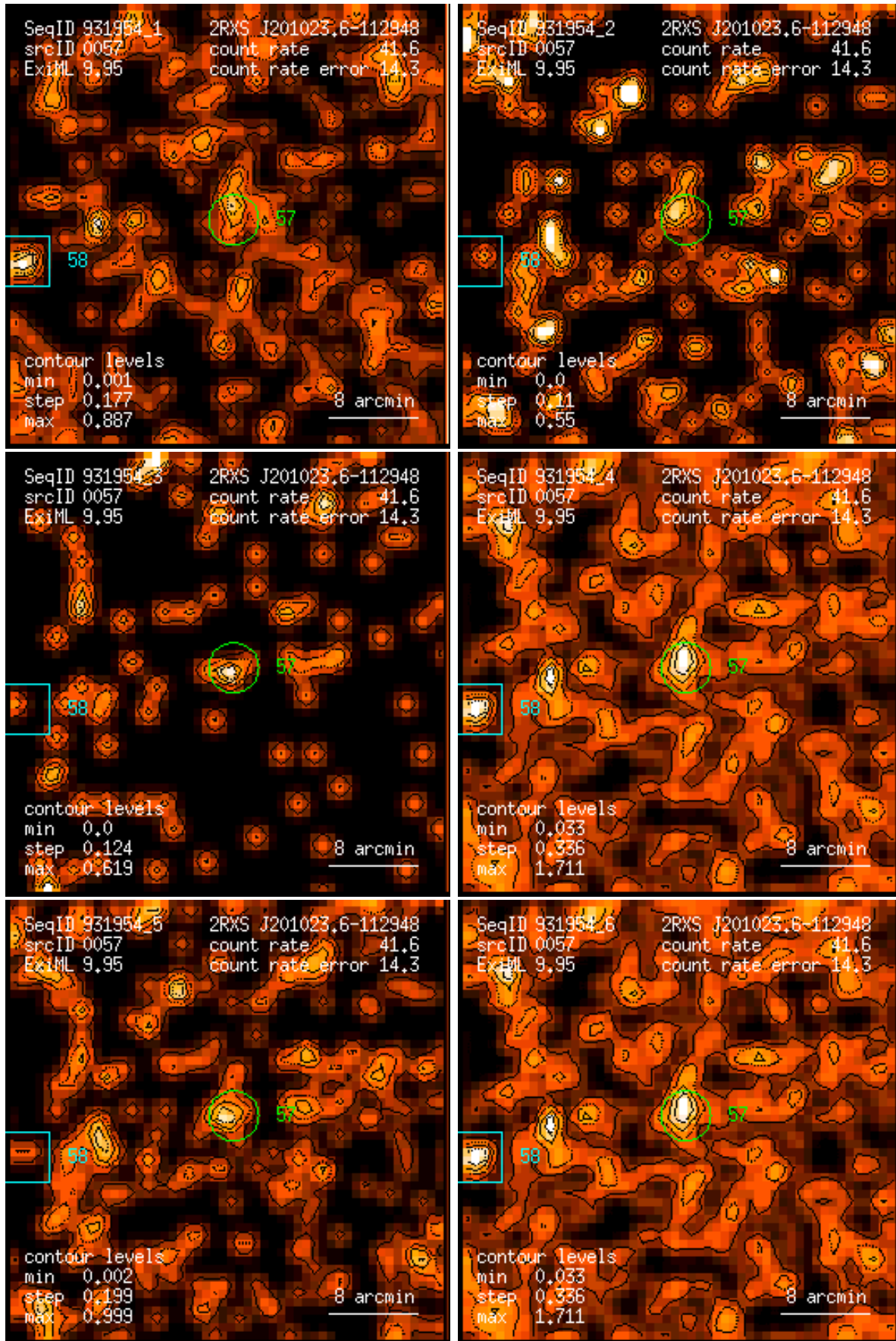
Figure 57: RASS 931954: detection 0057: band rate images, Gaussian filter: (1) PSPC channels 11 – 41, (2) 52 – 90, (3) 91 – 201, (4) 11 – 235, (5) 52 – 201, (6) 11 – 201. Broad band rates in counts/ks. Band rate contour levels in counts/ks/arcmin 2 .
