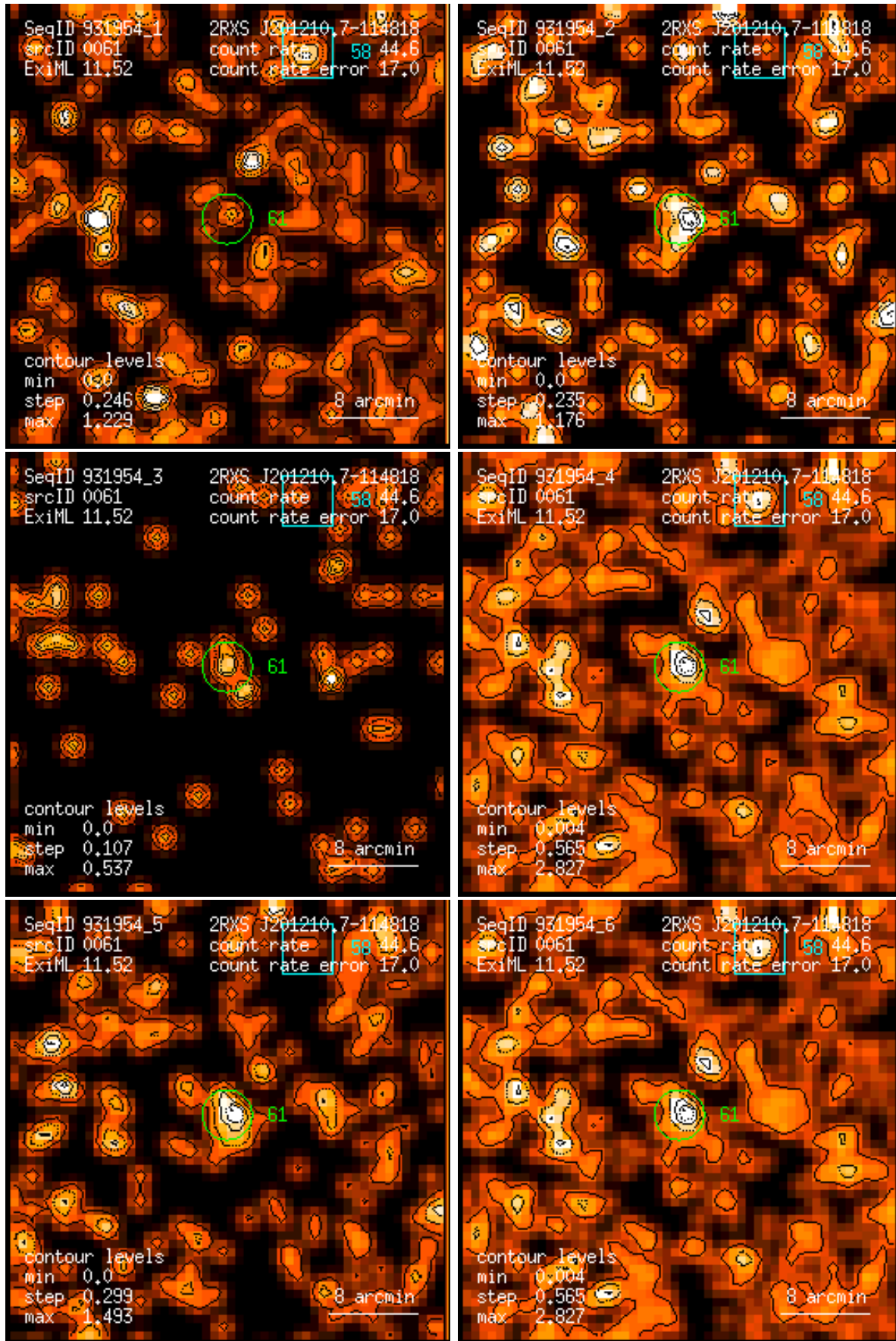
Figure 61: RASS 931954: detection 0061: band rate images, Gaussian filter: (1) PSPC channels 11 – 41, (2) 52 – 90, (3) 91 – 201, (4) 11 – 235, (5) 52 – 201, (6) 11 – 201. Broad band rates in counts/ks. Band rate contour levels in counts/ks/arcmin 2 .
