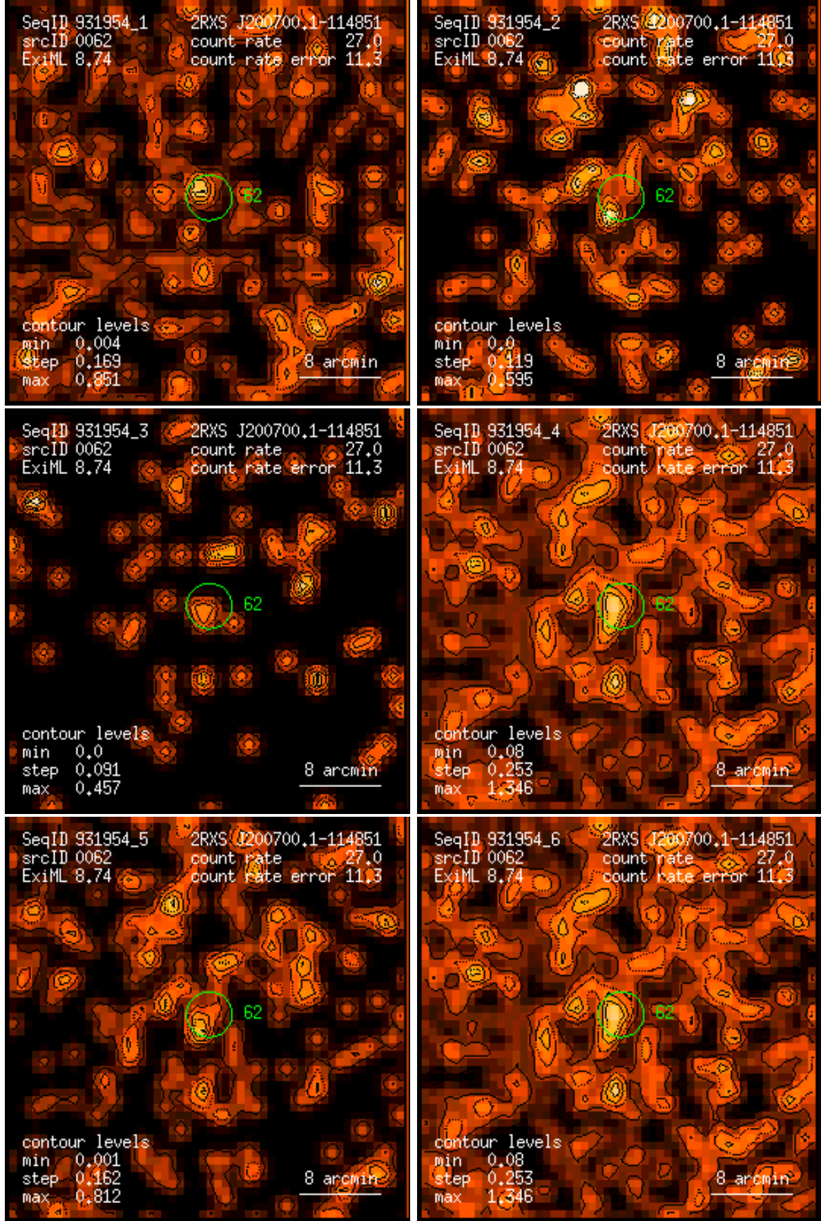
Figure 62: RASS 931954: detection 0062: band rate images, Gaussian filter: (1) PSPC channels 11 – 41, (2) 52 – 90, (3) 91 – 201, (4) 11 – 235, (5) 52 – 201, (6) 11 – 201. Broad band rates in counts/ks. Band rate contour levels in counts/ks/arcmin 2 .
