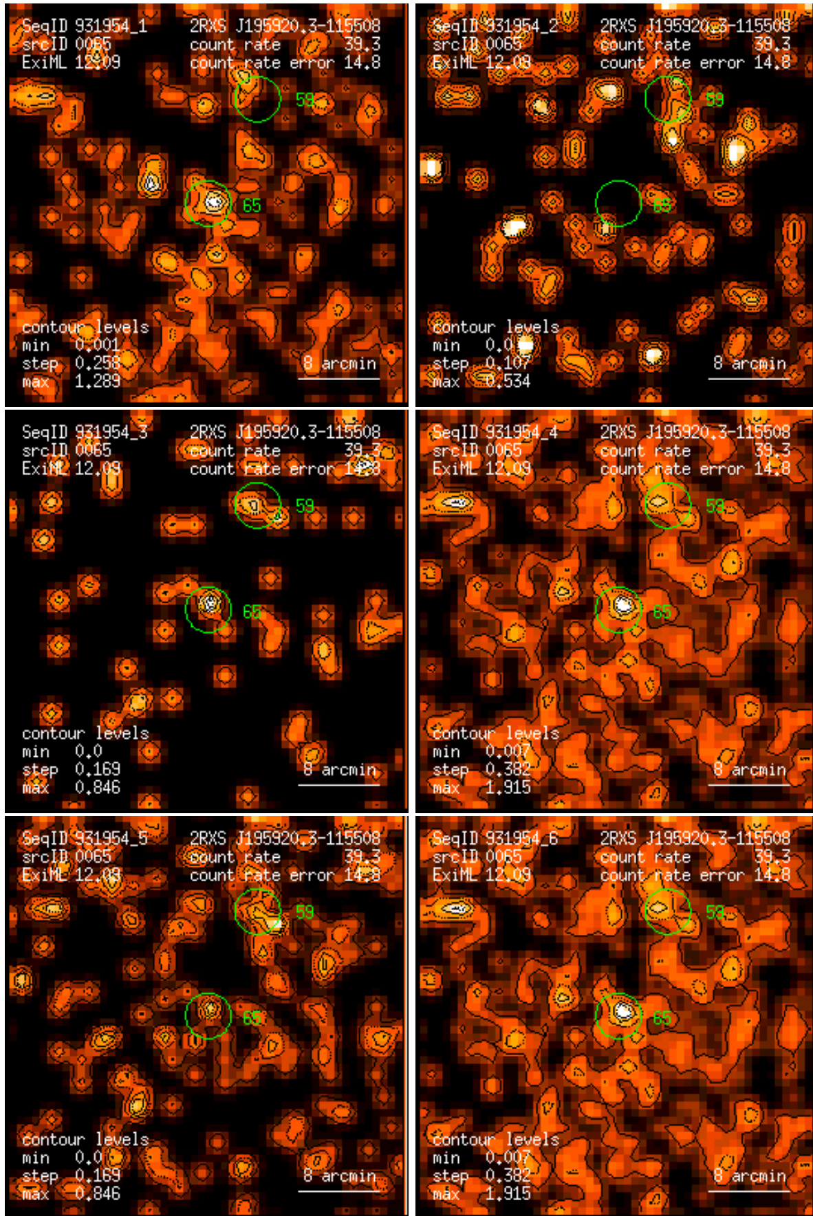
Figure 65: RASS 931954: detection 0065: band rate images, Gaussian filter: (1) PSPC channels 11 – 41, (2) 52 – 90, (3) 91 – 201, (4) 11 – 235, (5) 52 – 201, (6) 11 – 201. Broad band rates in counts/ks. Band rate contour levels in counts/ks/arcmin 2 .
