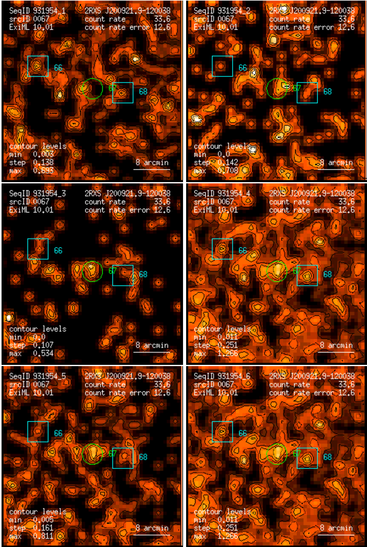
Figure 67: RASS 931954: detection 0067: band rate images, Gaussian filter: (1) PSPC channels 11 – 41, (2) 52 – 90, (3) 91 – 201, (4) 11 – 235, (5) 52 – 201, (6) 11 – 201. Broad band rates in counts/ks. Band rate contour levels in counts/ks/arcmin 2 .
